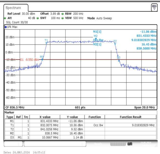
26(824-849)-10MHz-16QAM-26915-50RB#0-PASS
