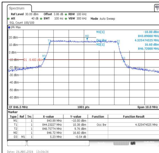
26(824-849)-5MHz-QPSK-27015-25RB#0-PASS
