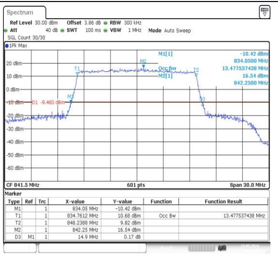
26(824-849)-15MHz-16QAM-26965-75RB#0-PASS
