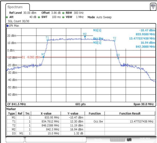
26(824-849)-15MHz-QPSK-26965-75RB#0-PASS
