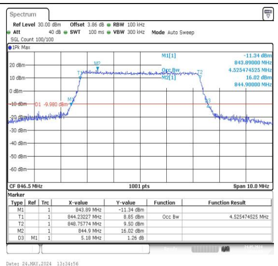
26(824-849)-5MHz-16QAM-27015-25RB#0-PASS
