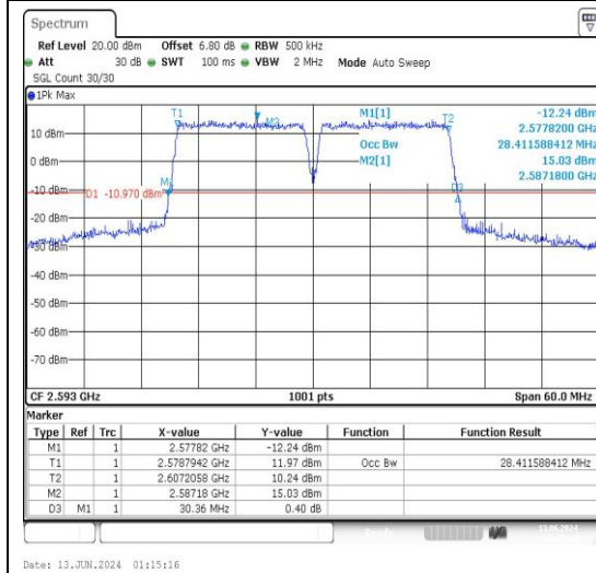
41-41-15MHz-15MHz-QPSK-QPSK-40545-40695 -75RB#0-75RB#0-PASS
