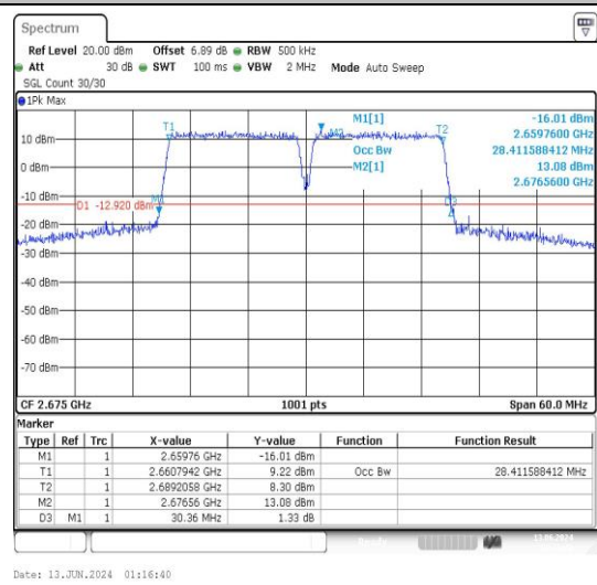
41-41-15MHz-15MHz-16QAM-16QAM-40545-4069 5-75RB#0-75RB#0-PASS
