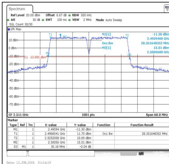
41-41-15MHz-15MHz-QPSK-QPSK-39725-39875 -75RB#0-75RB#0-PASS
