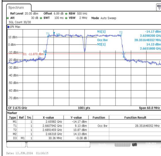
41-41-15MHz-15MHz-QPSK-QPSK-40545-40695 -75RB#0-75RB#0-PASS
