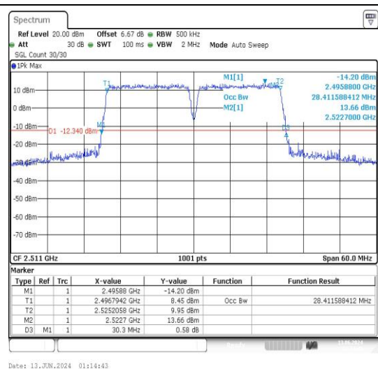
41-41-15MHz-15MHz-16QAM-16QAM-39725-3987 5-75RB#0-75RB#0-PASS
