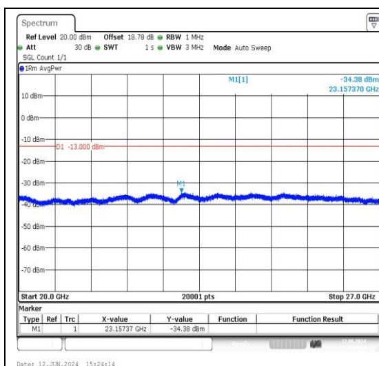
5-5-10MHz-5MHz-QPSK-QPSK-20450-20522-1R B#0-1RB#24-20000~27000MHz-PASS
