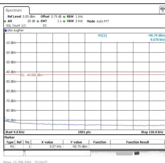
5-5-10MHz-5MHz-16QAM-16QAM-20450-20522-1 RB#0-1RB#24-0.009~0.15MHz-PASS
