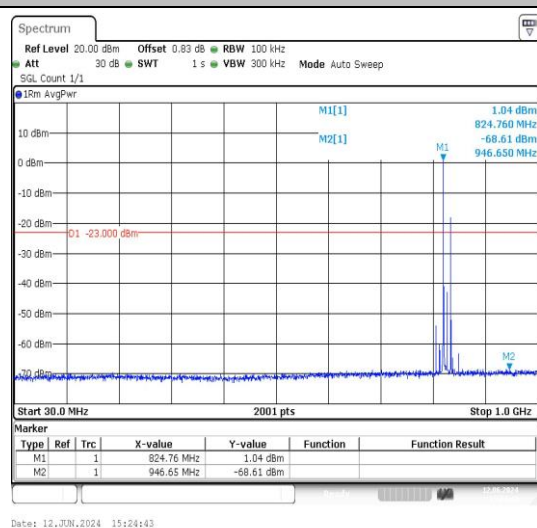
5-5-10MHz-5MHz-16QAM-16QAM-20450-20522-1 RB#0-1RB#24-30~1000MHz-PASS
