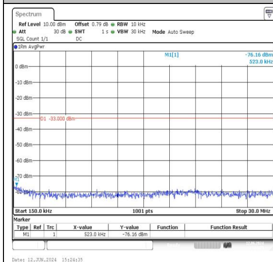
5-5-10MHz-5MHz-16QAM-16QAM-20450-20522-1 1RB#0-1RB#24-0.15~30MHz-PASS
