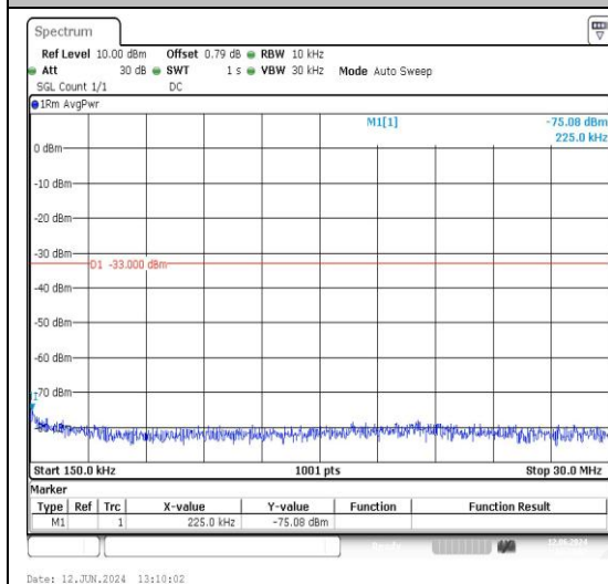
5-5-5MHz-10MHz-16QAM-16QAM-20428-20500-1 1RB#0-1RB#49-0.15~30MHz-PASS
