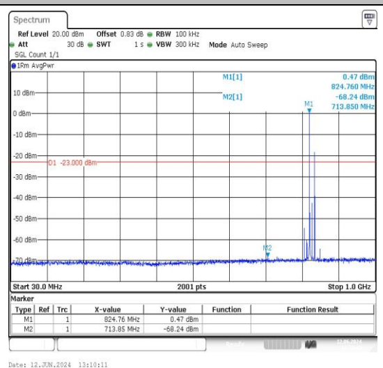
5-5-5MHz-10MHz-16QAM-16QAM-20428-20500-1 RB#0-1RB#49-30~1000MHz-PASS
