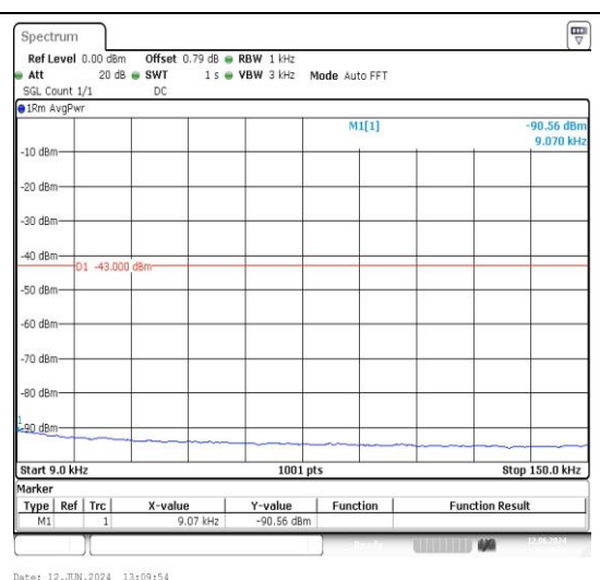
5-5-5MHz-10MHz-16QAM-16QAM-20428-20500-1 RB#0-1RB#49-0.009~0.15MHz-PASS
