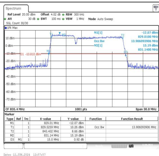
5-5-5MHz-10MHz-16QAM-16QAM-20478-20550-2 5RB#0-50RB#0-PASS
