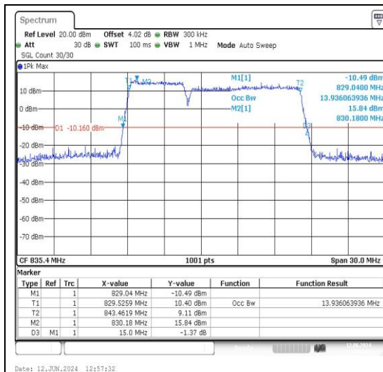
5-5-5MHz-10MHz-QPSK-QPSK-20478-20550-25 RB#0-50RB#0-PASS
