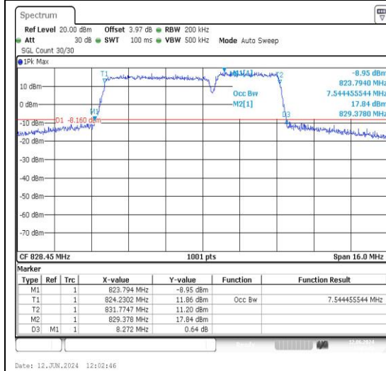
5-5-5MHz-3MHz-QPSK-QPSK-20425-20464-25R B#0-15RB#0-PASS
