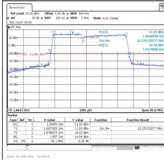
2-2-10MHz-15MHz-QPSK-QPSK-18653-18773-5 0RB#0-75RB#0-PASS
