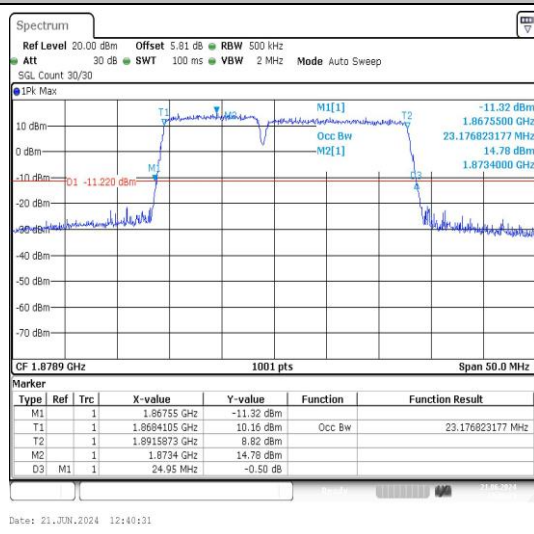
2-2-10MHz-15MHz-16QAM-16QAM-18653-18773- 50RB#0-75RB#0-PASS
