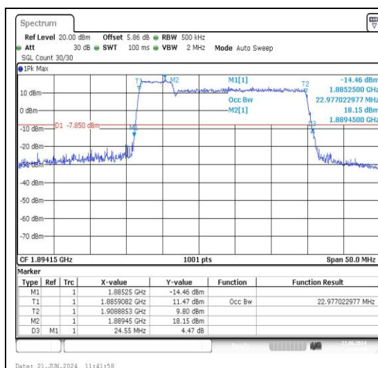
2-2-5MHz-20MHz-QPSK-QPSK-18983-19100-25 RB#0-100RB#0-PASS
