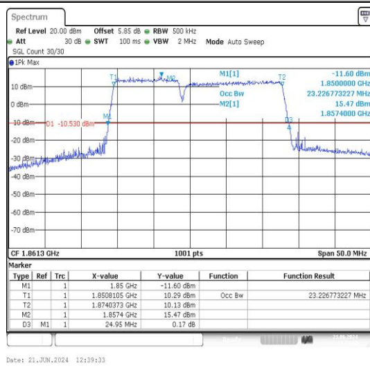
2-2-10MHz-15MHz-16QAM-16QAM-18653-18773- 50RB#0-75RB#0-PASS
