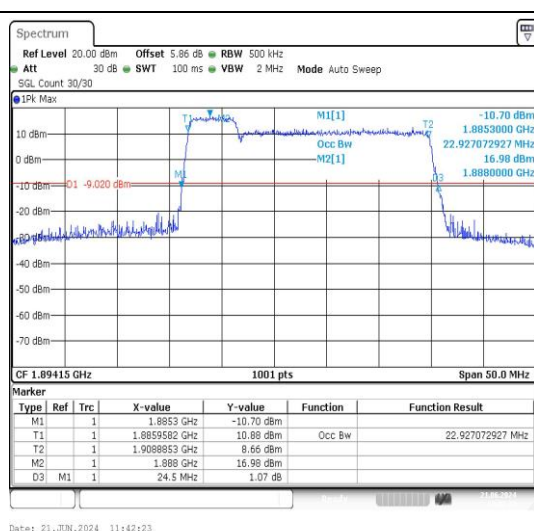
2-2-5MHz-20MHz-16QAM-16QAM-18983-19100-2 5RB#0-100RB#0-PASS
