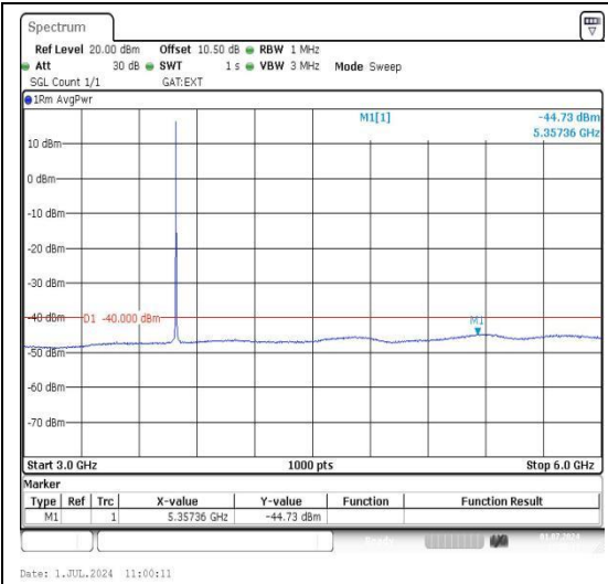
Band43_10MHz_QPSK_45540_1RB#0_3000~6000 00_3000~6000
