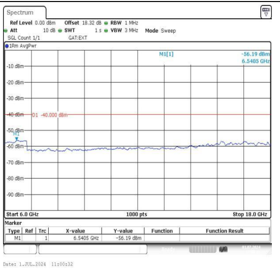
Band43_10MHz_QPSK_45540_1RB#0_6000~18000 00_6000~18000
