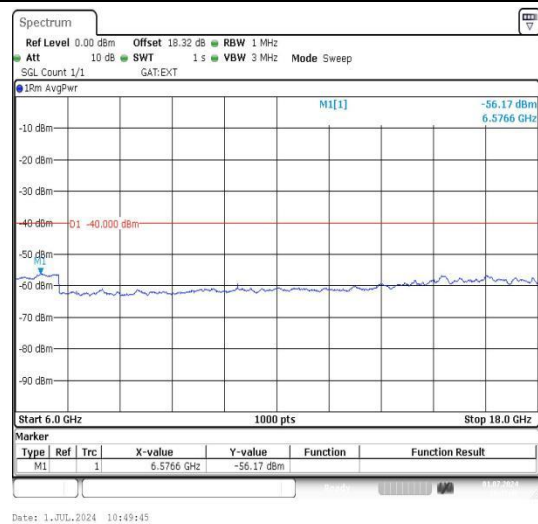
Band43_10MHz_QPSK_44640_1RB#0_6000~18000_00_6000~18000
