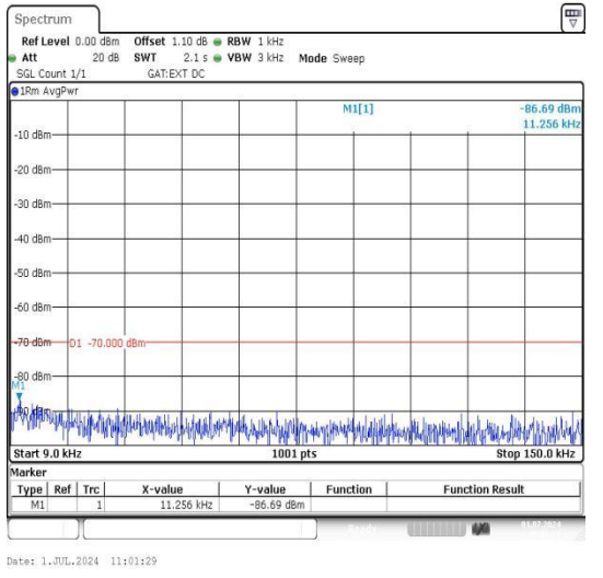
Band43_10MHz_16QAM_45540_1RB#0_0.009~0.15 15_0.009~0.15
