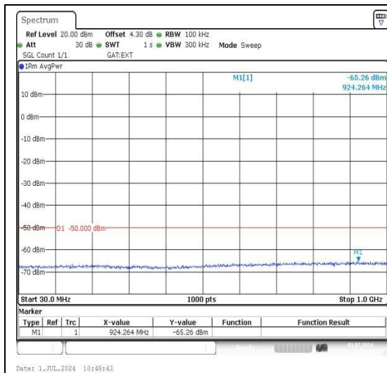
Band43_10MHz_QPSK_44640_1RB#0_30~1000_30~1000
