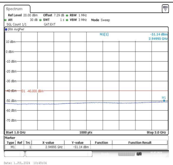
Band43_10MHz_QPSK_44640_1RB#0_1000~3000_0_1000~3000
