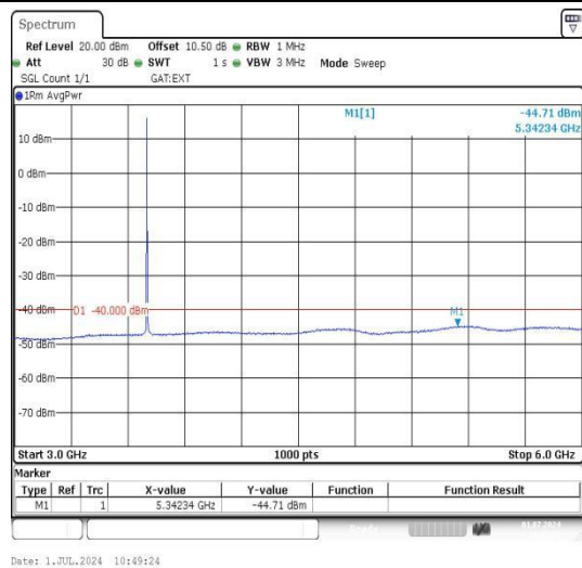
Band43_10MHz_QPSK_44640_1RB#0_3000~6000_00_3000~6000
