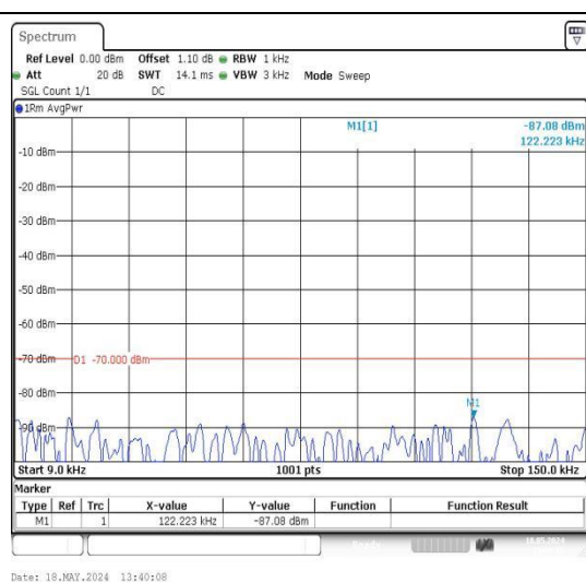
Band30_5MHz_16QAM_27710_1RB#0_0.009~0.15_0.009~0.15
