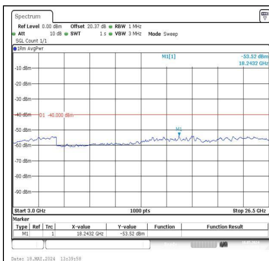
Band30_5MHz_QPSK_27710_1RB#0_3000~26500_3000~26500
