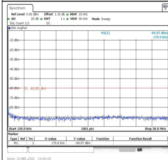
Band30_5MHz_16QAM_27710_1RB#0_0.15~30_0.15~30
