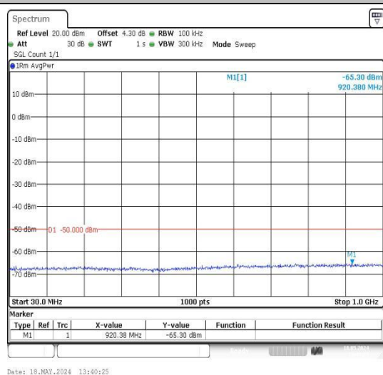
Band30_5MHz_16QAM_27710_1RB#0_30~1000_30~1000
