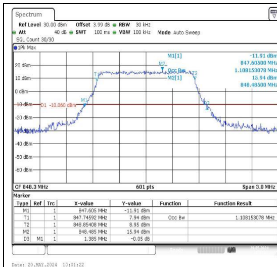
26(824-849)-1.4MHz-QPSK-27033-6RB#0-PASS
