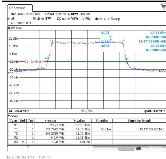
26(824-849)-15MHz-QPSK-26915-75RB#0-PASS
