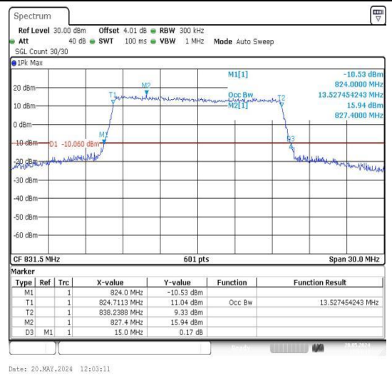
26(824-849)-15MHz-16QAM-26865-75RB#0-PASS
