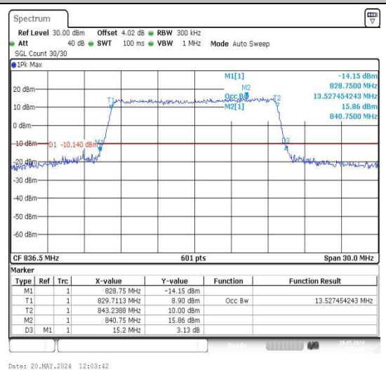
26(824-849)-15MHz-16QAM-26915-75RB#0-PASS
