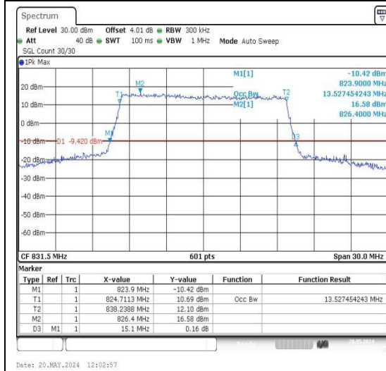
26(824-849)-15MHz-QPSK-26865-75RB#0-PASS
