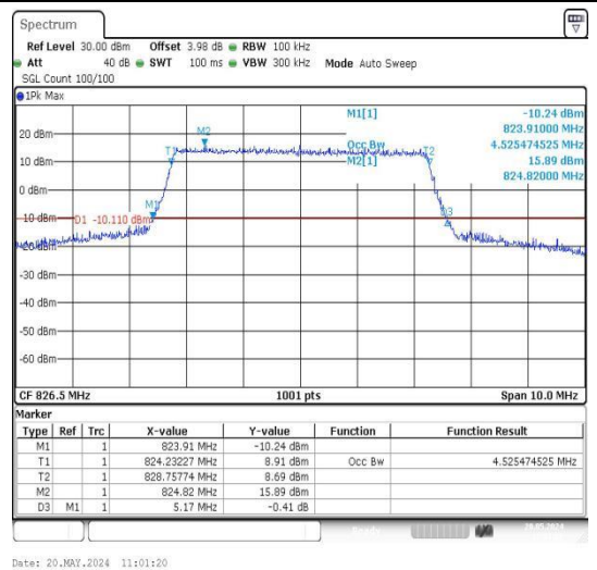
26(824-849)-5MHz-16QAM-26815-25RB#0-PASS
