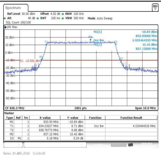
26(824-849)-5MHz-16QAM-26915-25RB#0-PASS
