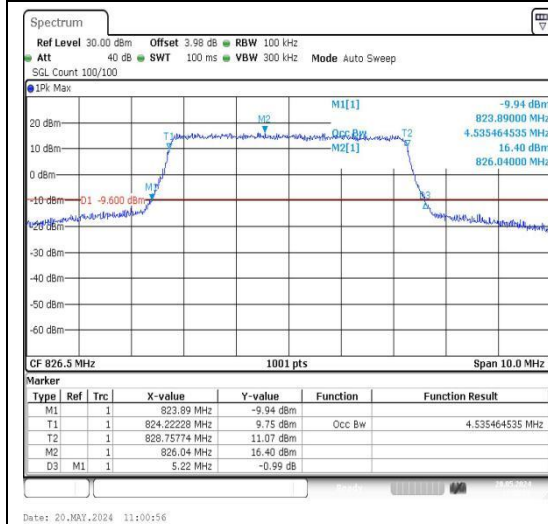
26(824-849)-5MHz-QPSK-26815-25RB#0-PASS
