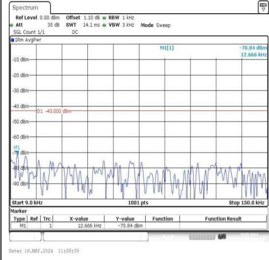
Band25_10MHz_QPSK_26365_1RB#0_0.009~0.15_0.009~0.15
