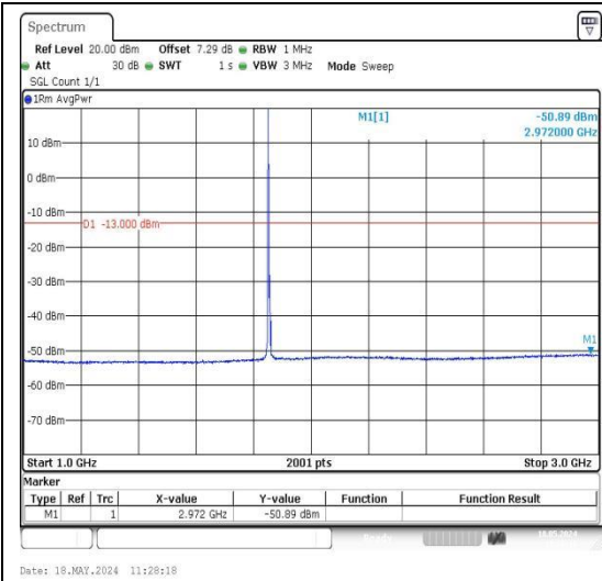
Band25_10MHz_16QAM_26090_1RB#0_1000~3000_1000~3000
