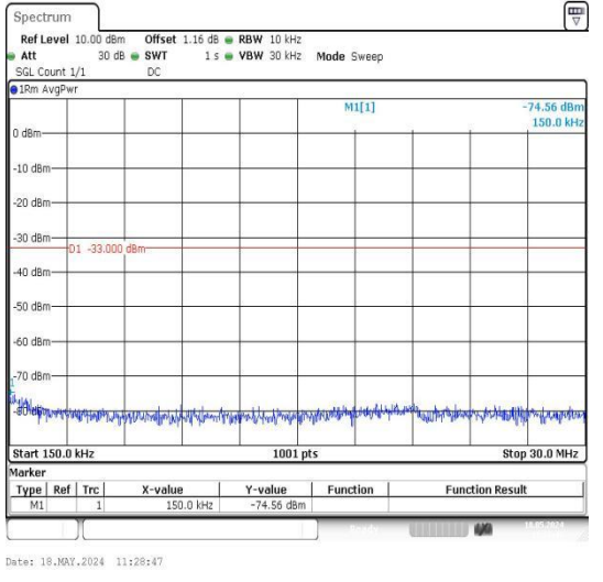
Band25_10MHz_QPSK_26365_1RB#0_0.15~30_0.15~30
