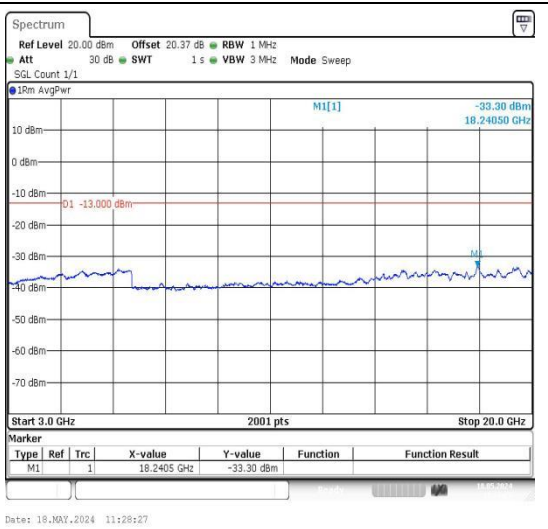
Band25_10MHz_16QAM_26090_1RB#0_3000~20000_3000~20000
