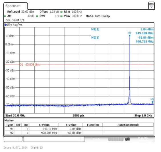
5-5-10MHz-5MHz-16QAM-16QAM-20550-20622-1
