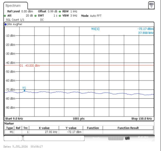
5-5-10MHz-5MHz-16QAM-16QAM-20550-20622-1 RB#49-ORB#0-0.009~0.15MHz-PASS
