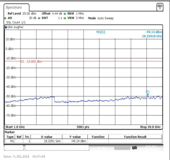
5-5-10MHz-5MHz-QPSK-QPSK-20550-20622-1RB #49-ORB#0-1000~20000MHz-PASS
