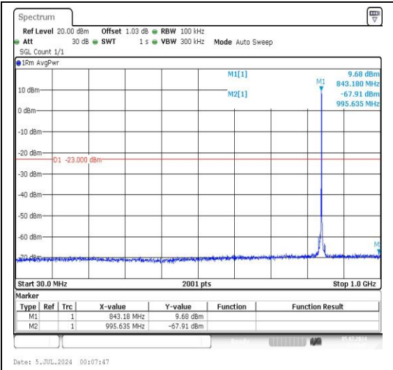
5-5-10MHz-5MHz-QPSK-QPSK-20550-20622-1R B#49-ORB#0-30~1000MHz-PASS
