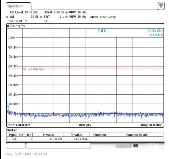
5-5-10MHz-5MHz-16QAM-16QAM-20550-20622-
