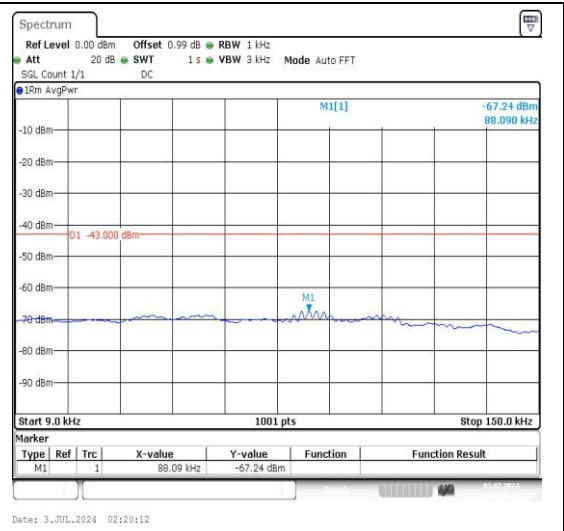
2-2-20MHz-5MHz-16QAM-16QAM-19050-19167-1 RB#0-1RB#24-0.009~0.15MHz-PASS
