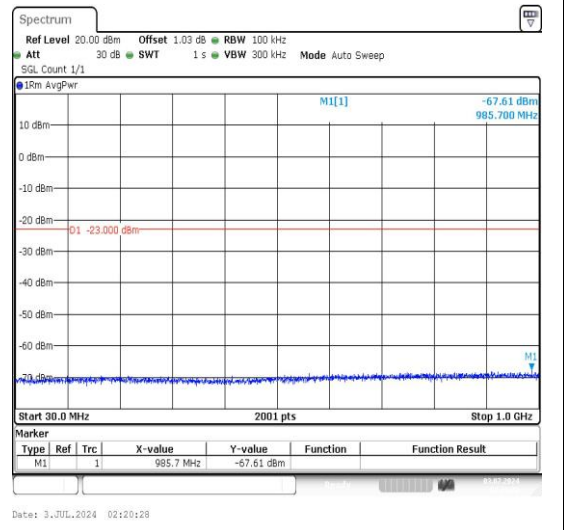
2-2-20MHz-5MHz-16QAM-16QAM-19050-19167-1 RB#0-1RB#24-30~1000MHz-PASS
