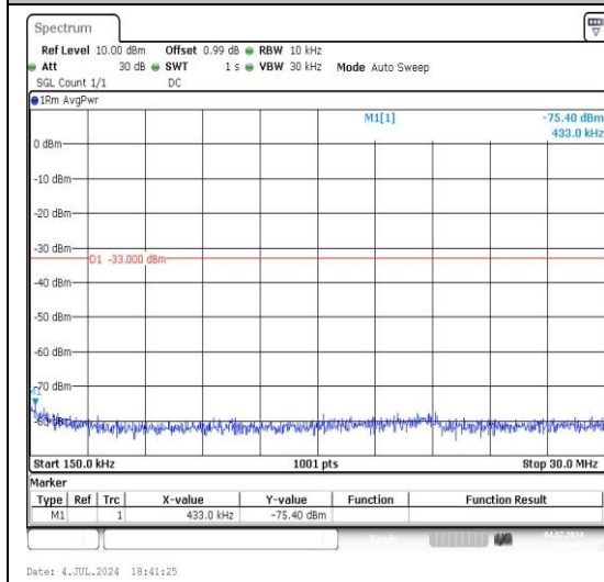
5-5-5MHz-3MHz-16QAM-16QAM-20425-20464-1
