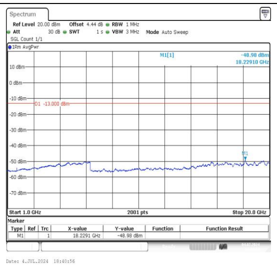
5-5-5MHz-3MHz-QPSK-QPSK-20425-20464-1RB# 24-ORB#0-1000~20000MHz-PASS
