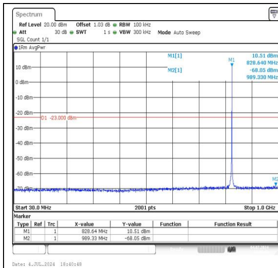
5-5-5MHz-3MHz-QPSK-QPSK-20425-20464-1RB #24-ORB#0-30~1000MHz-PASS
