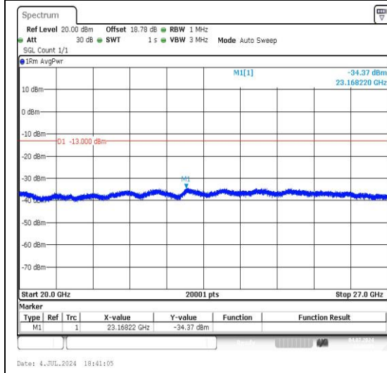
5-5-5MHz-3MHz-QPSK-QPSK-20425-20464-1RB #24-ORB#0-20000~27000MHz-PASS
