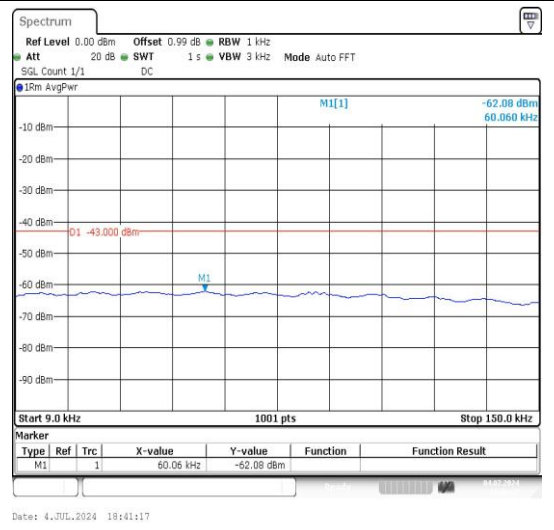
5-5-5MHz-3MHz-16QAM-16QAM-20425-20464-1R B#24-ORB#0-0.009~0.15MHz-PASS
