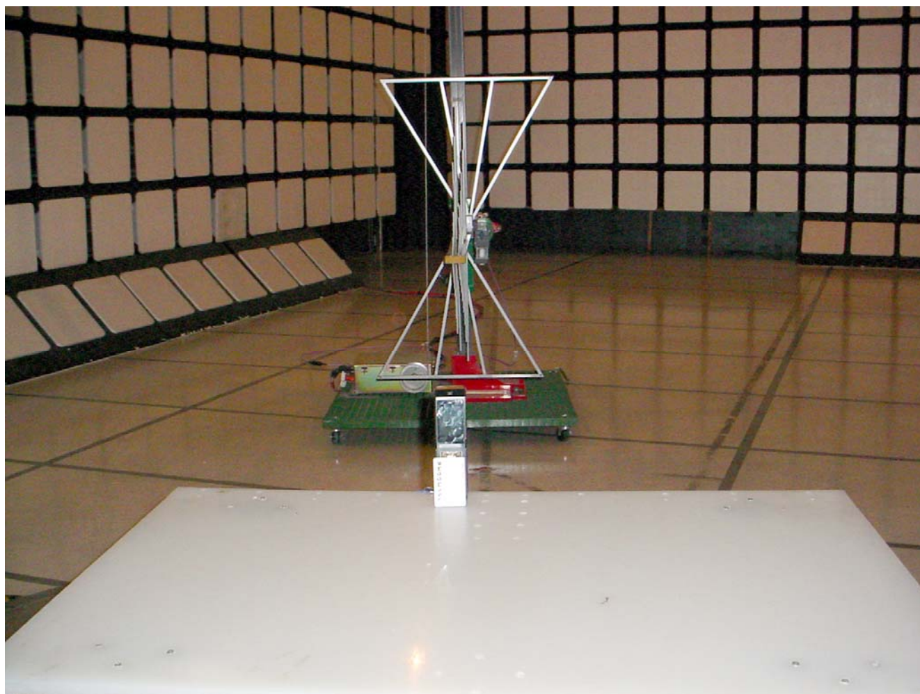
Radiated Emissions at 3 m Distance (Above 30 MHz)
