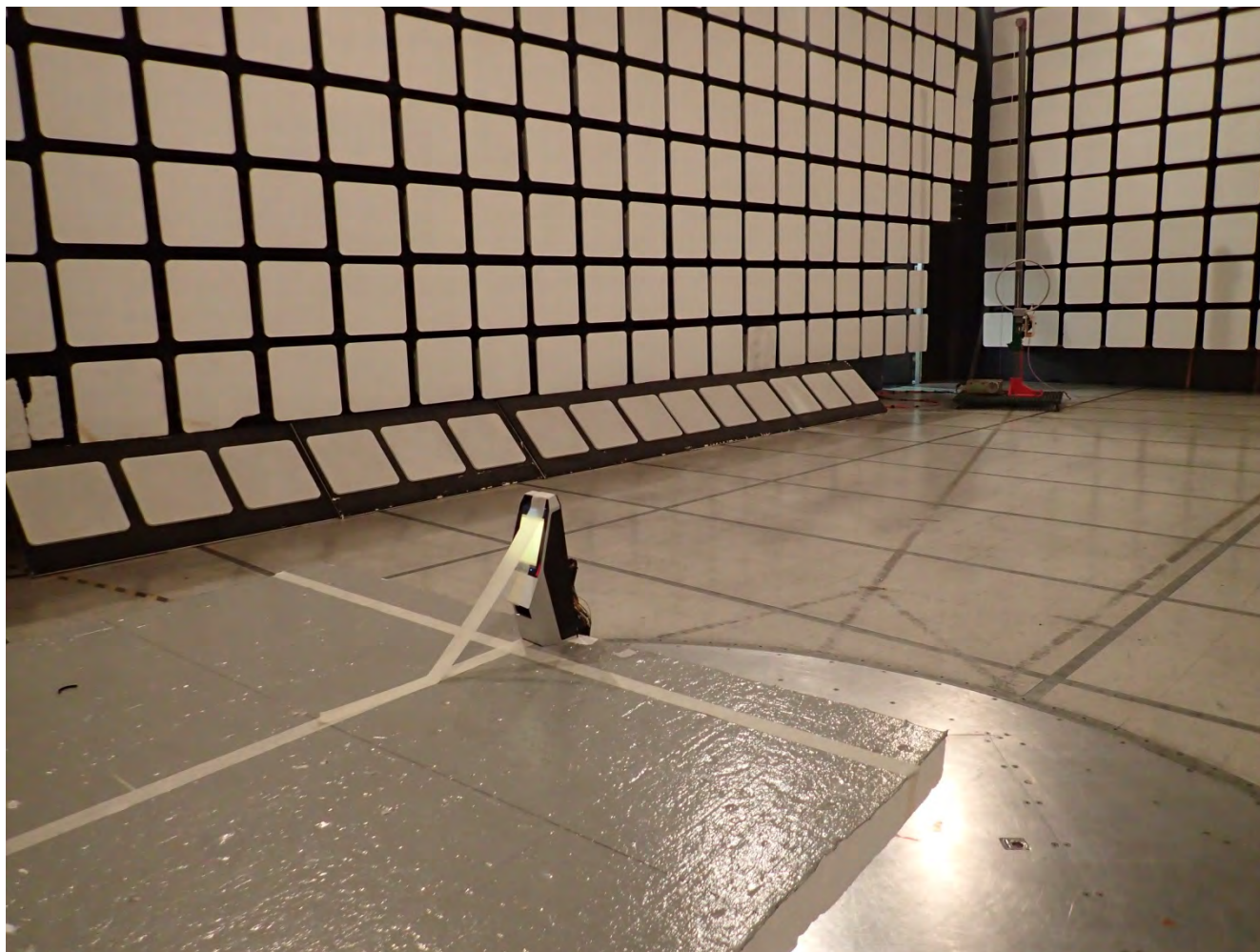
Radiated Emissions at 10 m Distance (for frequencies below 30 MHz)
