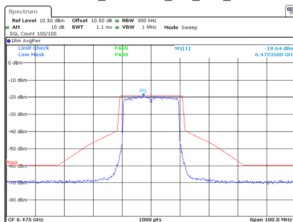
802.11ax20_6475MHz_RU_Full_ANT 1
