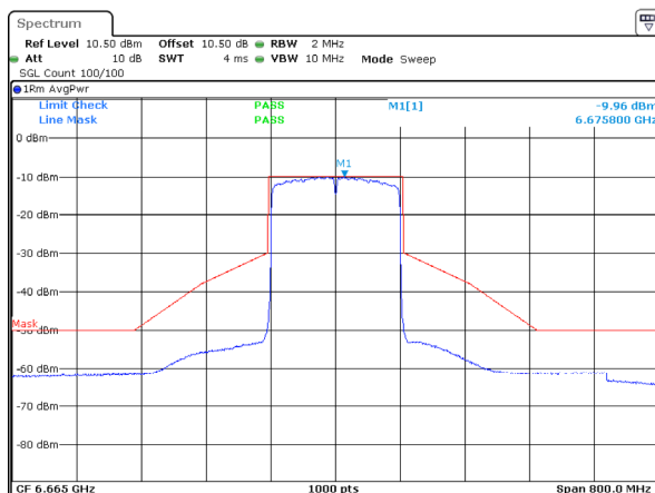
802.11ax160_6665MHz_RU_Full_ANT 1
