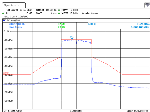
802.11ax160_6825MHz_RU_Full_ANT 2
