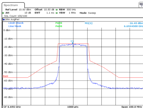
802.11ax20_6695MHz_RU_Full_ANT 1
