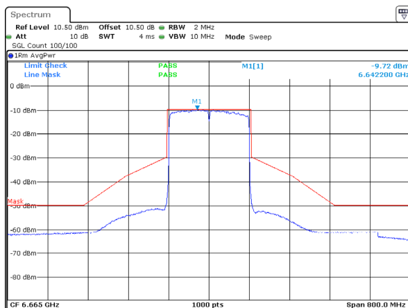
802.11ax160_6665MHz_RU_Full_ANT 2
