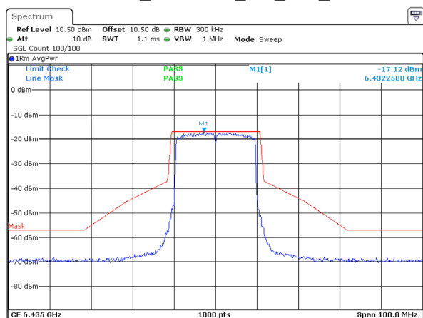
802.11ax20_6435MHz_RU_Full_ANT 1
