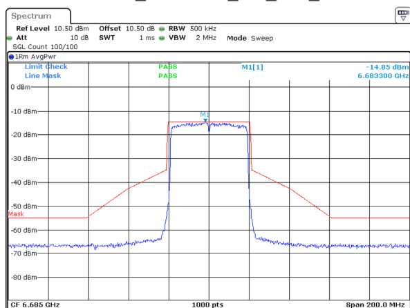
802.11ax40_6685MHz_RU_Full_ANT 2
