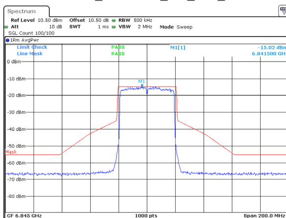
802.11ax40_6845MHz_RU_Full_ANT 2
