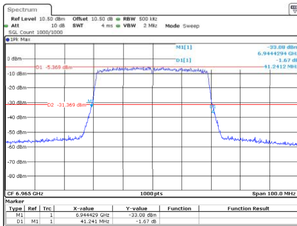
802.11ax40_6965MHz_RU_Full_ANT2 41.241MHz
