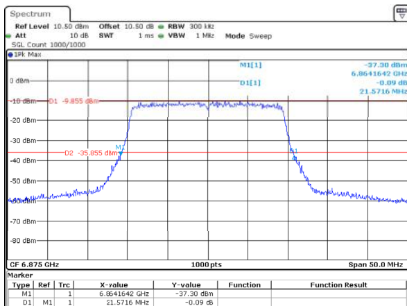
802.11ax20_6875MHz_RU_Full_ANT1 21.572MHz
