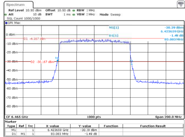
802.11ax80_6465MHz_RU_Full_ANT1 83.083MHz
