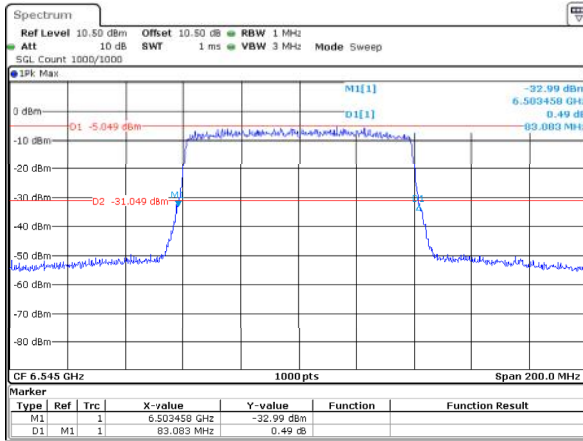
802.11ax80_6545MHz_RU_Full_ANT1 83.083MHz
