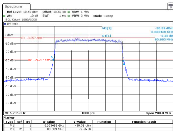
802.11ax80_6705MHz_RU_Full_ANT2 83.083MHz
