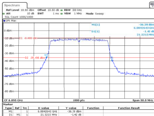
802.11ax20_6895MHz_RU_Full_ANT1 21.522MHz
