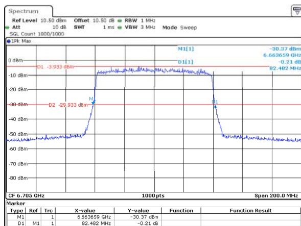
802.11ax80_6705MHz_RU_Full_ANT1 82.482MHz
