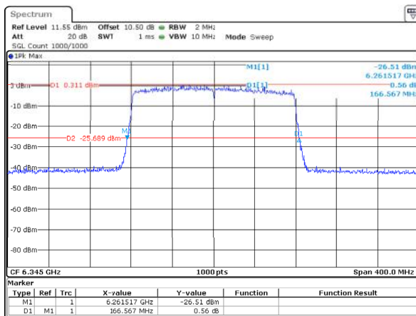
802.11ax160_6345MHz_RU_Full_ANT1 166.567MHz
