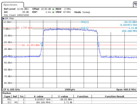
802.11ax160_6185MHz_RU_Full_ANT2 166.166MHz
