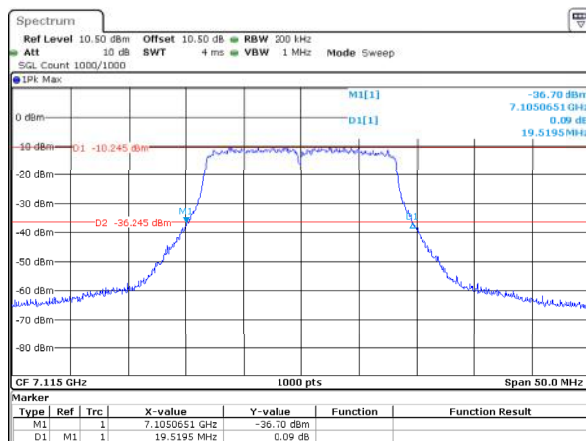
802.11a_7115MHz_ANT2 19.520MHz
