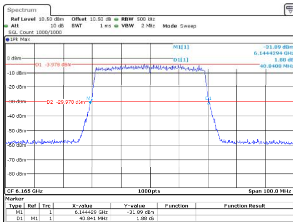
802.11ax40_6165MHz_RU_Full_ANT2 40.841MHz
