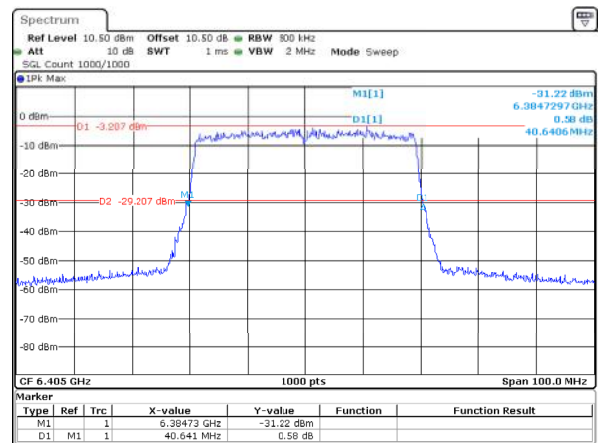
802.11ax40_6405MHz_RU_Full_ANT2 40.641MHz
