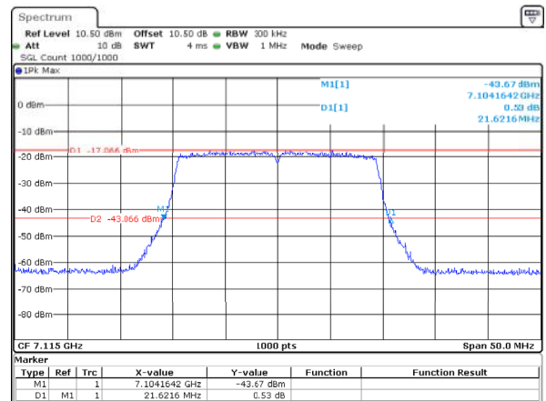
802.11ax20_7115MHz_RU_Full_ANT1 21.622MHz
