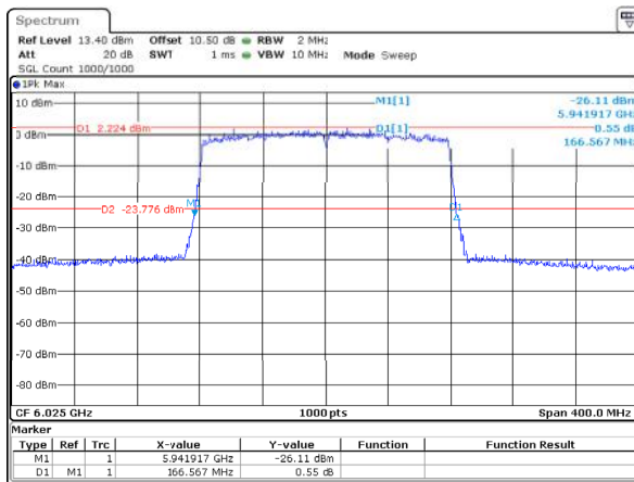
802.11ax160_6025MHz_RU_Full_ANT1 166.567MHz
