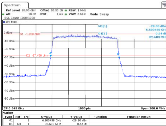
802.11ax80_6545MHz_RU_Full_ANT2 82.683MHz
