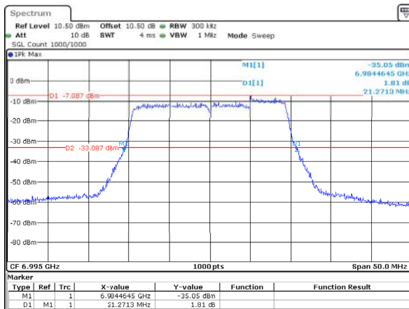
802.11ax20_6995MHz_RU_Full_ANT1 21.271MHz
