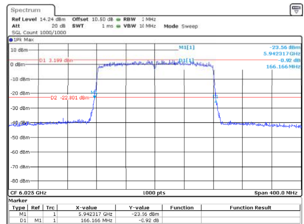
802.11ax160_6025MHz_RU_Full_ANT2 166.166MHz
