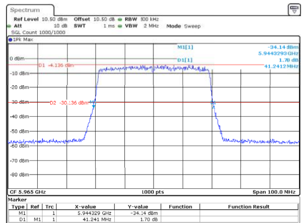
802.11ax40_5965MHz_RU_Full_ANT2 41.241MHz
