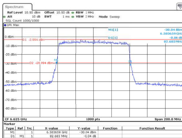
802.11ax80_6625MHz_RU_Full_ANT2 82.683MHz
