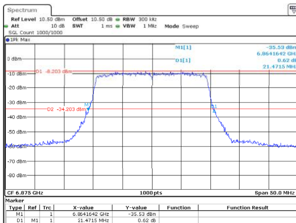
802.11ax20_6875MHz_RU_Full_ANT2 21.471MHz
