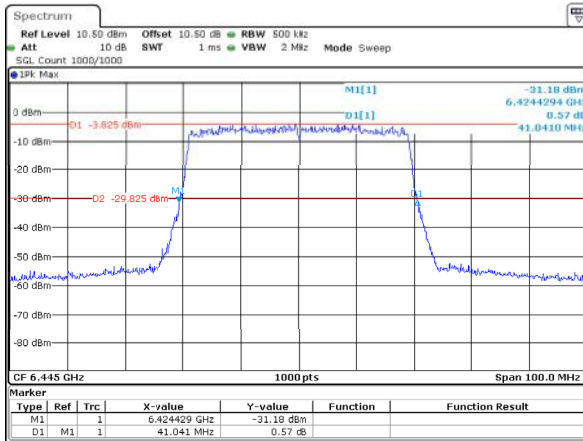
802.11ax40_6445MHz_RU_Full_ANT2 41.041MHz
