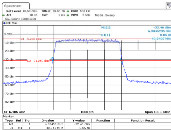
802.11ax40_6405MHz_RU_Full_ANT1 40.841MHz
