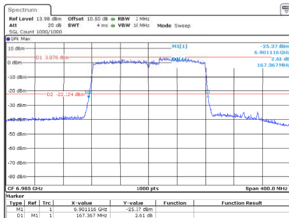
802.11ax160_6985MHz_RU_Full_ANT2 167.367MHz
