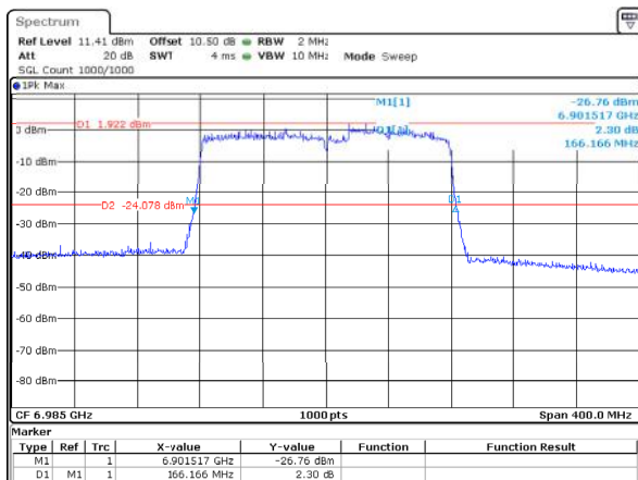
802.11ax160_6985MHz_RU_Full_ANT1 166.166MHz
