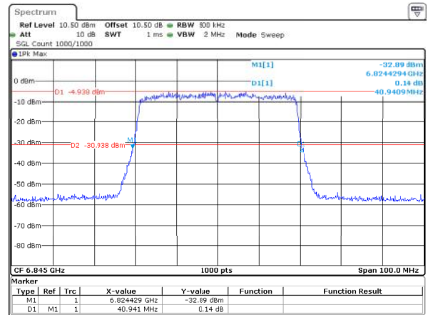
802.11ax40_6845MHz_RU_Full_ANT2 40.941MHz
