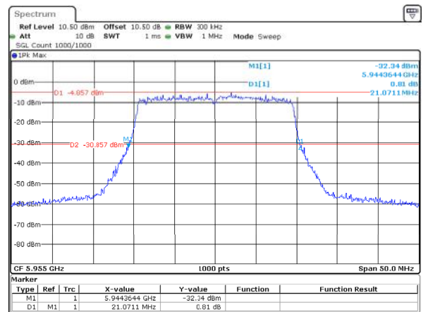
802.11ax20_5955MHz_RU_Full_ANT2 21.071MHz
