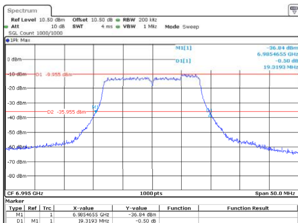
802.11a_6995MHz_ANT2 19.319MHz
