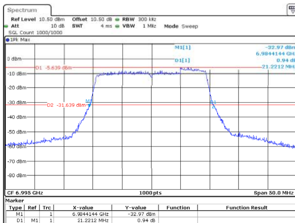
802.11ax20_6995MHz_RU_Full_ANT2 21.221MHz
