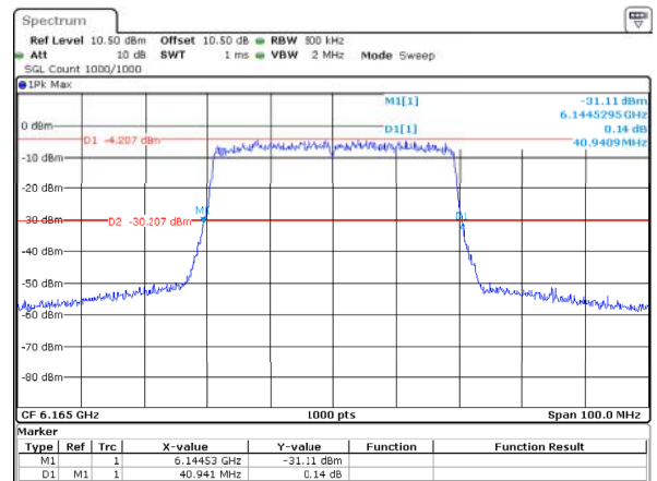
802.11ax40_6165MHz_RU_Full_ANT1 40.941MHz
