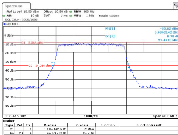
802.11ax20_6415MHz_RU_Full_ANT1 21.471MHz
