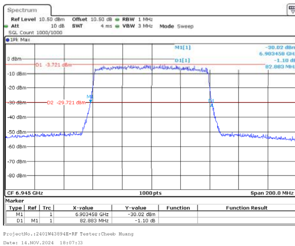
802.11ax80_6945MHz_RU_Full_ANT2 82.883MHz
