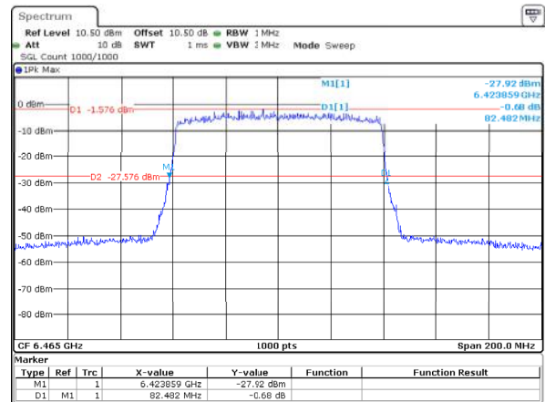
802.11ax80_6465MHz_RU_Full_ANT2 82.482MHz
