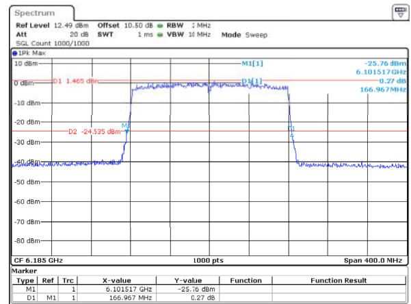
802.11ax160_6185MHz_RU_Full_ANT1 166.967MHz
