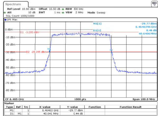
802.11ax40_6485MHz_RU_Full_ANT2 40.641MHz
