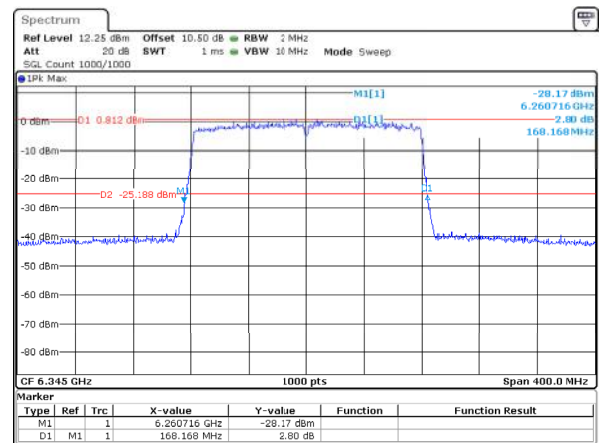
802.11ax160_6345MHz_RU_Full_ANT2 168.168MHz
