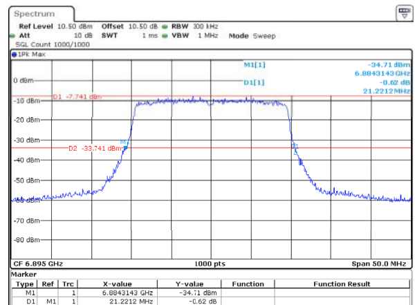
802.11ax20_6895MHz_RU_Full_ANT2 21.221MHz
