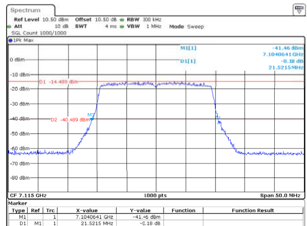
802.11ax20_7115MHz_RU_Full_ANT2 21.522MHz
