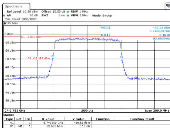
802.11ax80_6785MHz_RU_Full_ANT2 82.683MHz
