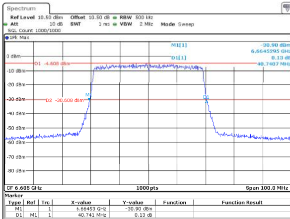
802.11ax40_6685MHz_RU_Full_ANT2 40.741MHz
