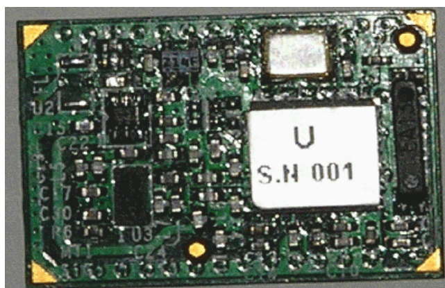
Figure 1 PCB Side 1
