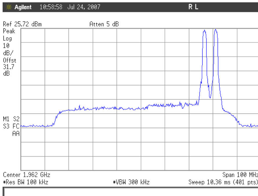
CDMA Intermodulation, Downlink High End
