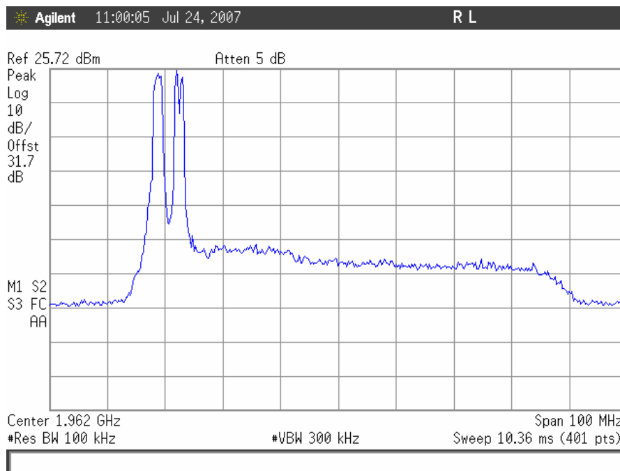
CDMA Intermodulation, Downlink Low End
