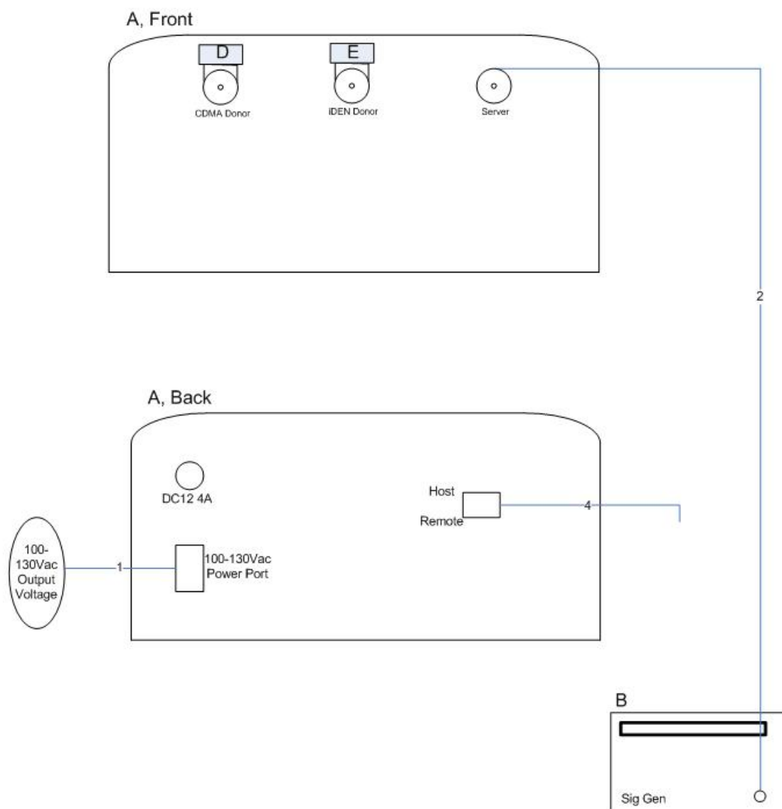
Figure 2. Block Diagram of Test Configuration (Spurious Emissions – Uplink)
