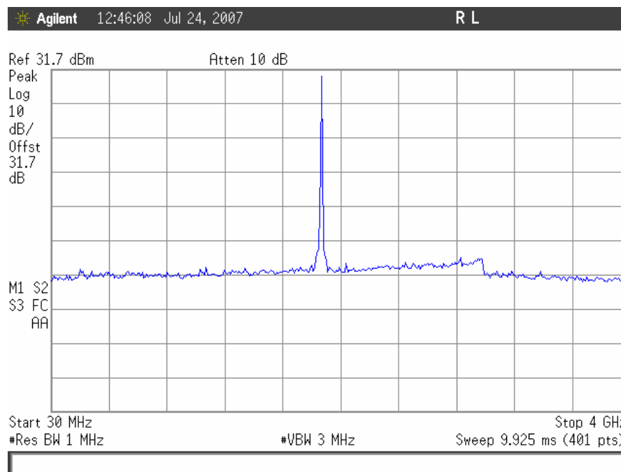
Conducted Spurious Emissions, CDMA Mid Channel Downlink, 30MHz – 4GHz
