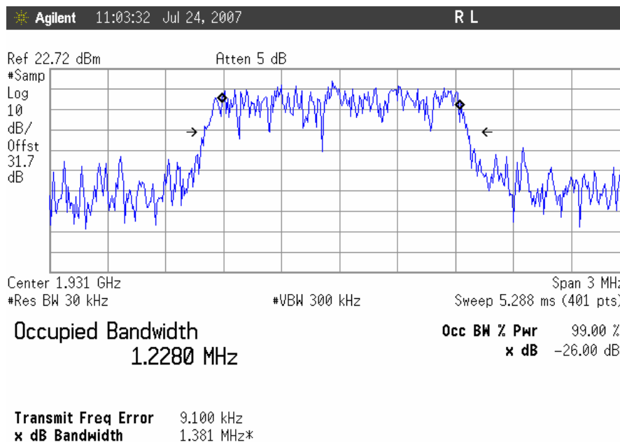
Occupied Bandwidth, CDMA Downlink, Low Channel Output
