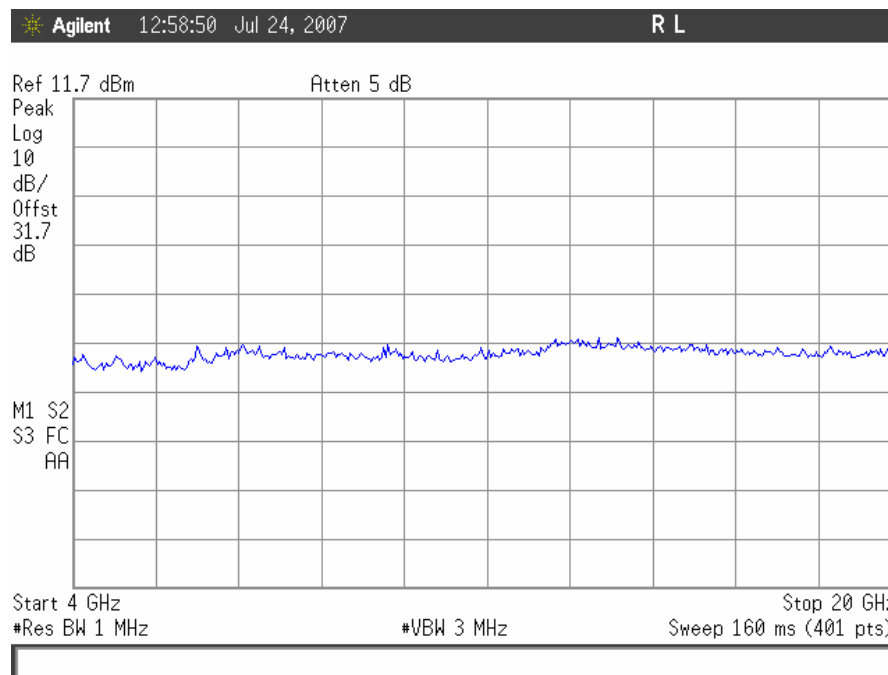
Conducted Spurious Emissions, CDMA High Channel Downlink, 4GHz – 20GHz
