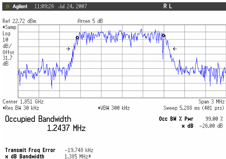
Occupied Bandwidth, CDMA Uplink, Low Channel Output
