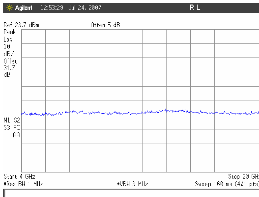
Conducted Spurious Emissions, CDMA Low Channel Downlink, 4GHz – 20GHz
