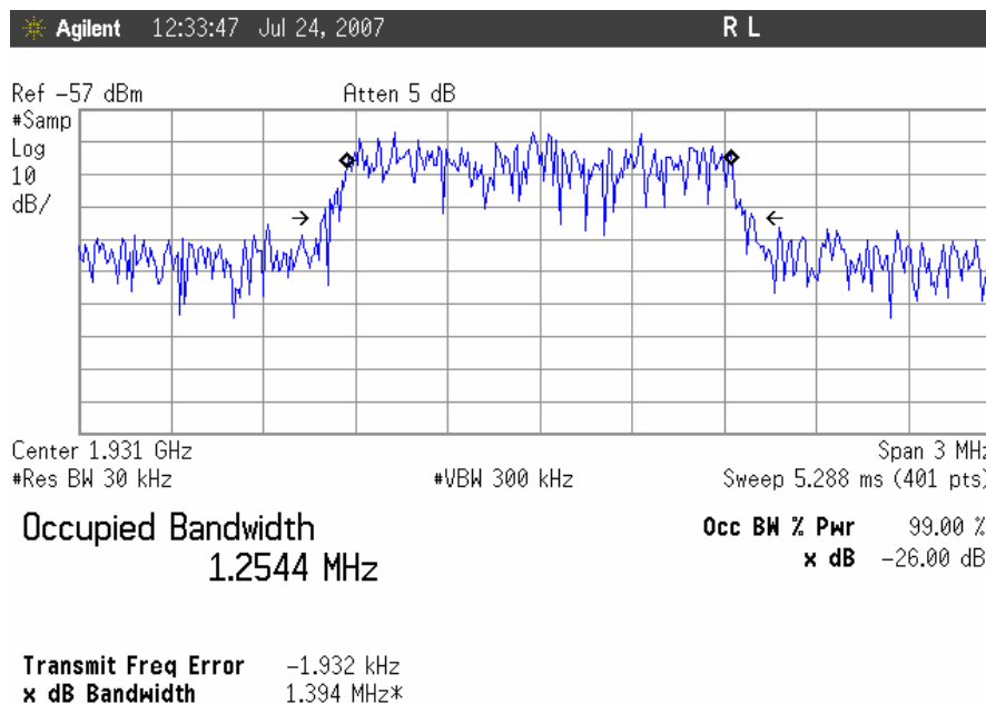
Occupied Bandwidth, CDMA Downlink, Low Channel Input
