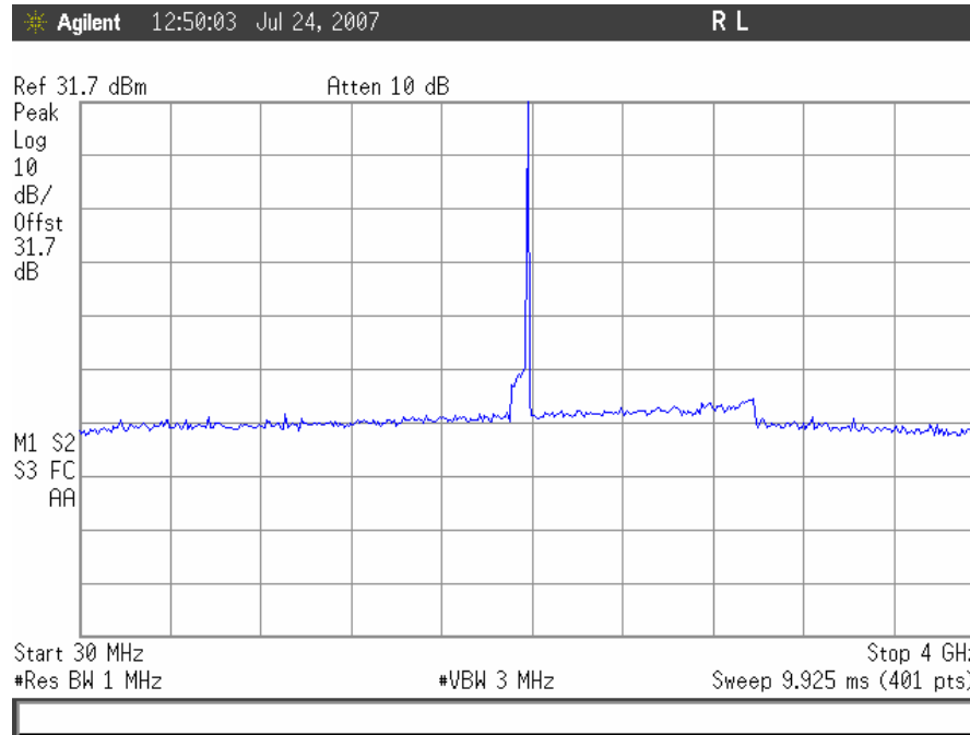
Conducted Spurious Emissions, CDMA High Channel Downlink, 30MHz – 4GHz
