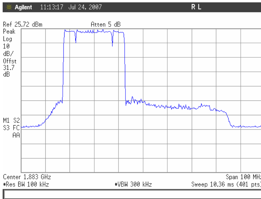
Out of Band Rejection, Uplink, Low End, 15MHz
