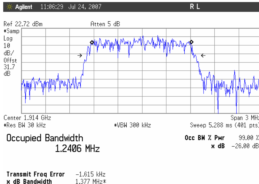
Occupied Bandwidth, CDMA Uplink, High Channel Output
