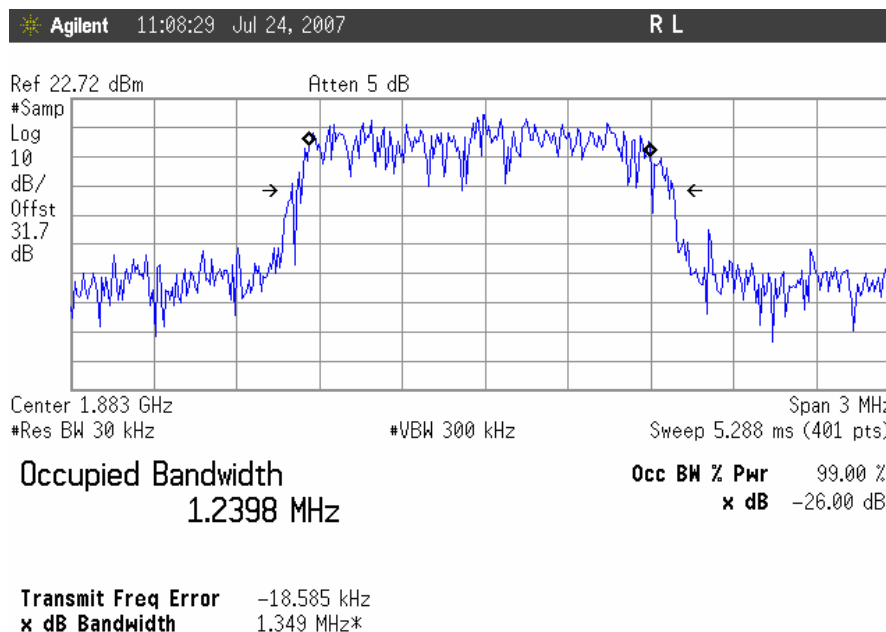
Occupied Bandwidth, CDMA Uplink, Mid Channel Output
