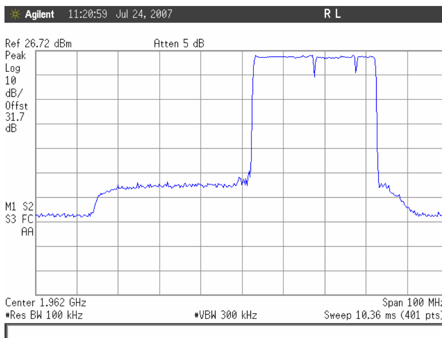
Out of Band Rejection, Downlink, High End, 15MHz
