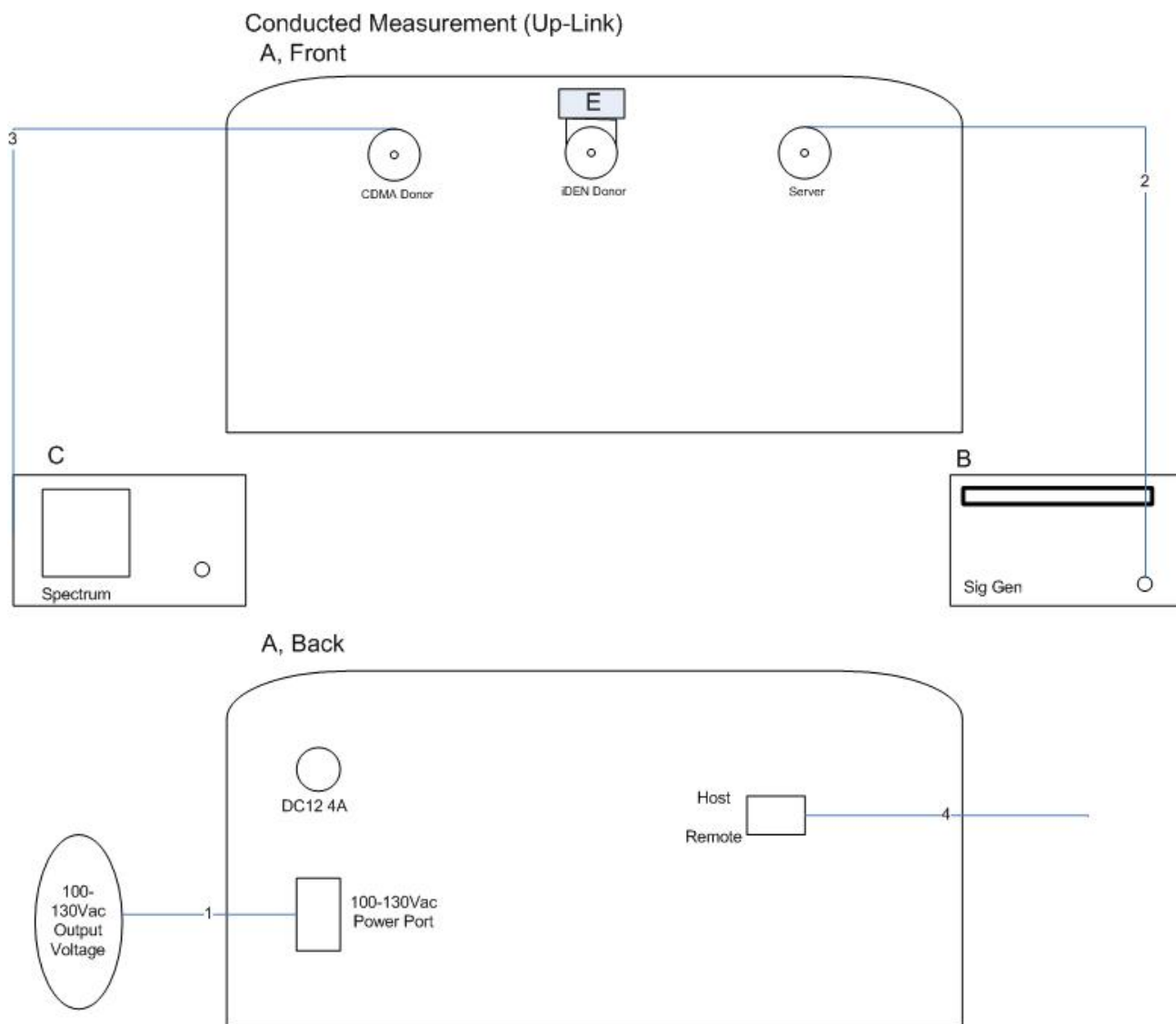
Figure 4. Block Diagram of Test Configuration (Conducted Measurement – Uplink)
