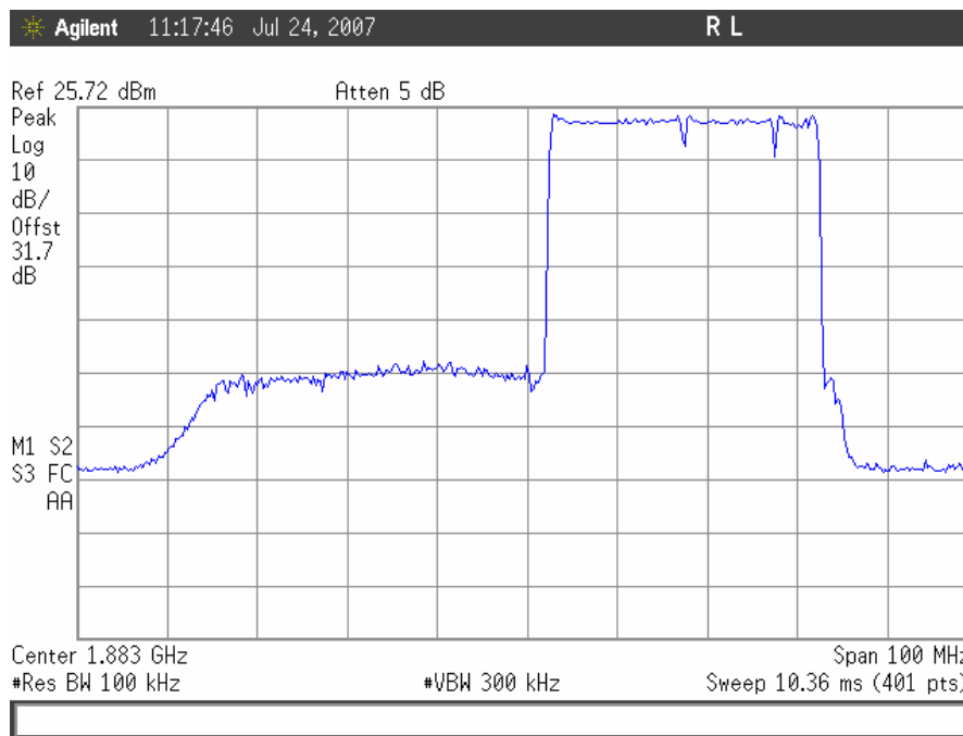
Out of Band Rejection, Uplink, High End, 15MHz
