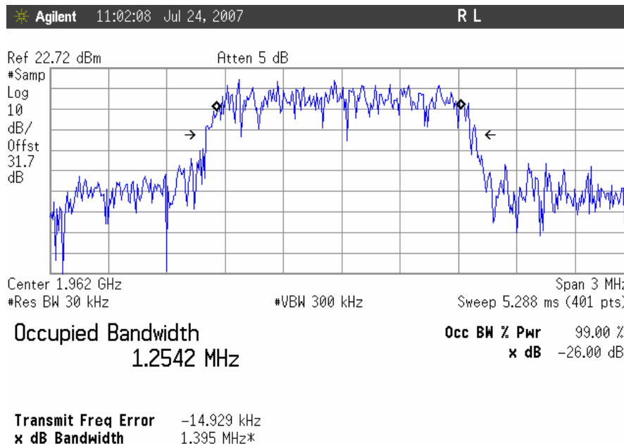
Occupied Bandwidth, CDMA Downlink, Mid Channel Output
