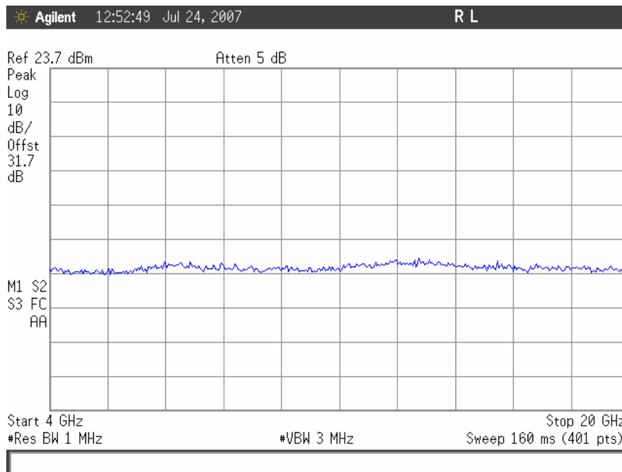
Conducted Spurious Emissions, CDMA Mid Channel Downlink, 4GHz – 20GHz
