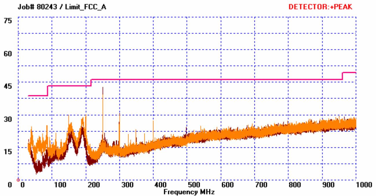
Plot 3. Radiated Emissions 30MHz – 1GHz Plot
