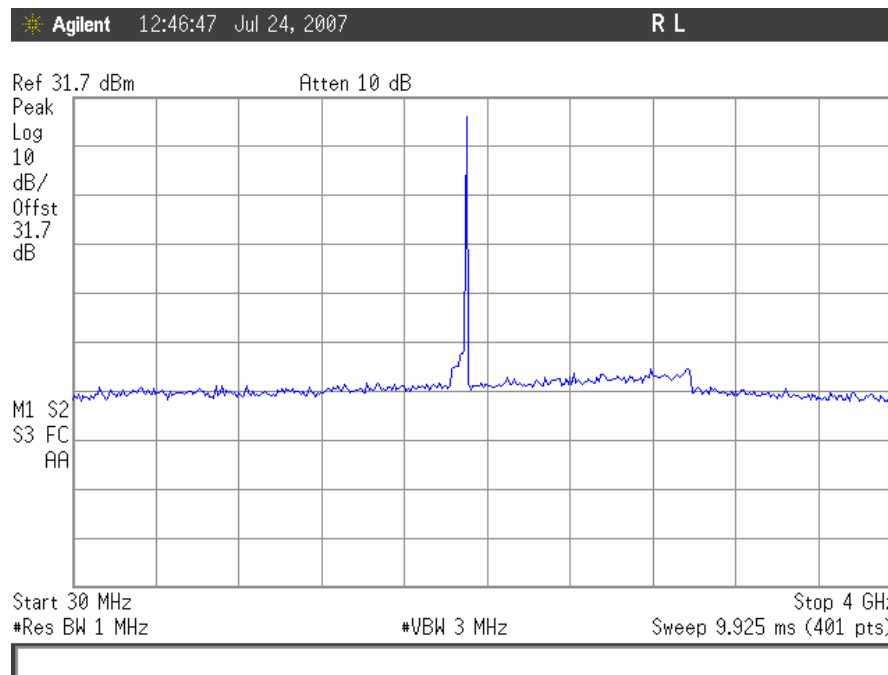
Conducted Spurious Emissions, CDMA High Channel Downlink, 30MHz – 4GHz
