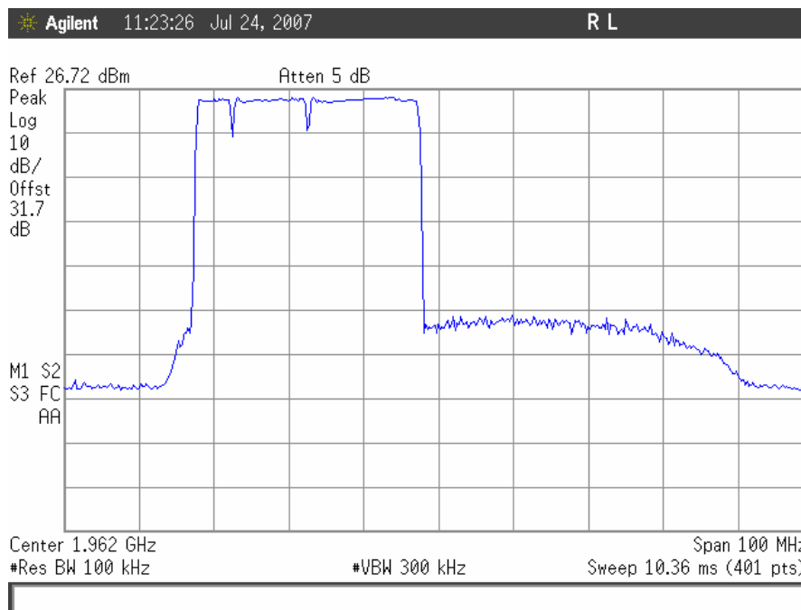
Out of Band Rejection, Downlink, Low End, 15MHz
