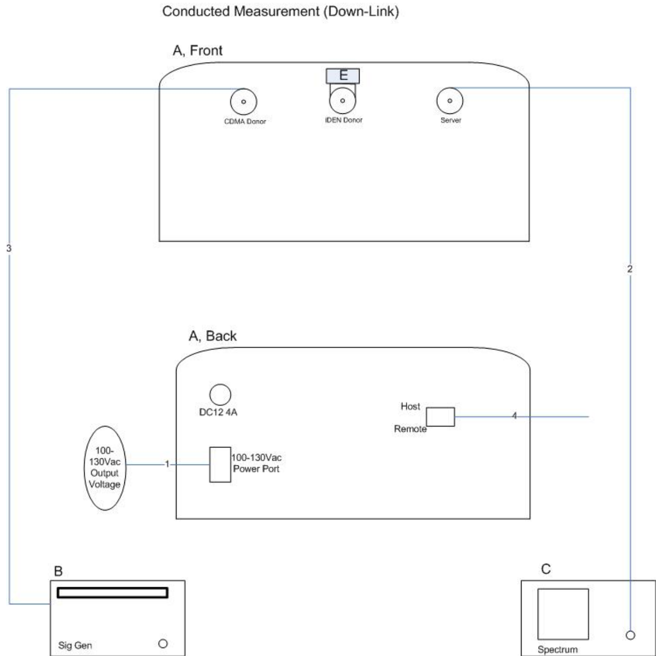
Figure 3. Block Diagram of Test Configuration (Conducted Measurement - Downlink)
