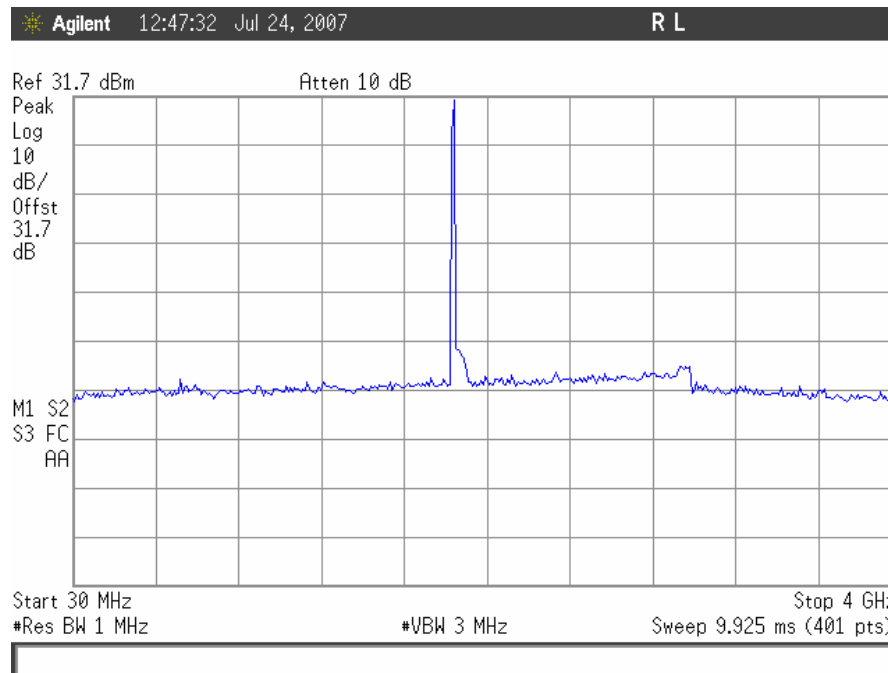
Conducted Spurious Emissions, CDMA Low Channel Downlink, 30MHz – 4GHz
