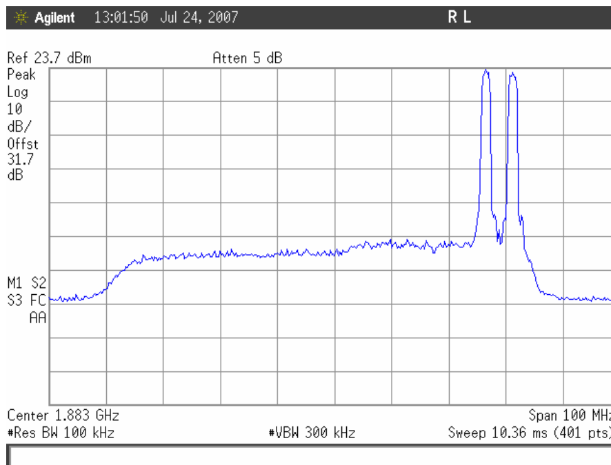
CDMA Intermodulation, Uplink High End
