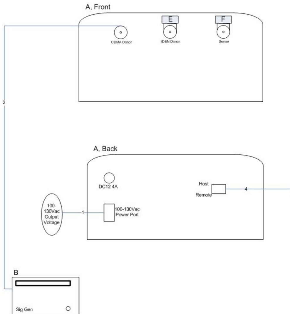
Figure 1. Block Diagram of Test Configuration (Spurious Emissions - Downlink)
