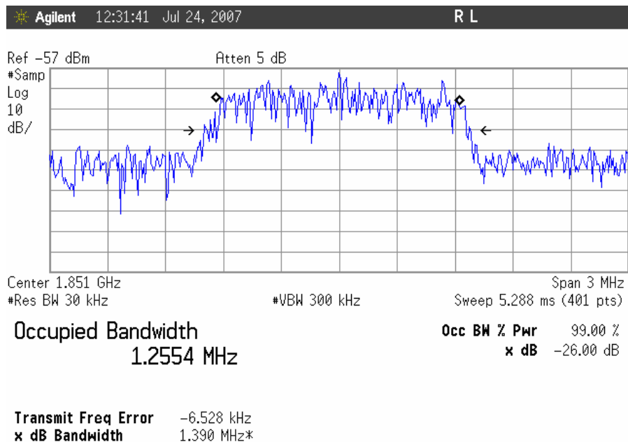
Occupied Bandwidth, CDMA Uplink, Low Channel Input
