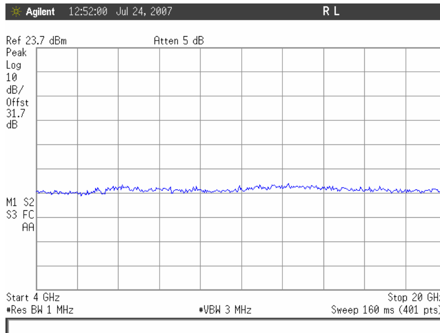
Conducted Spurious Emissions, CDMA High Channel Downlink, 4GHz – 20GHz
