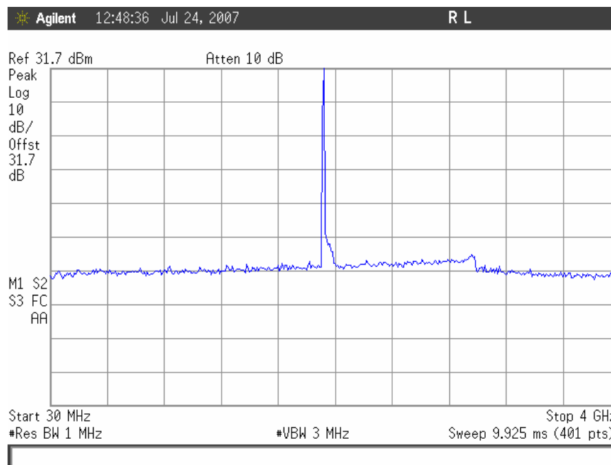
Conducted Spurious Emissions, CDMA Low Channel Downlink, 30MHz – 4GHz
