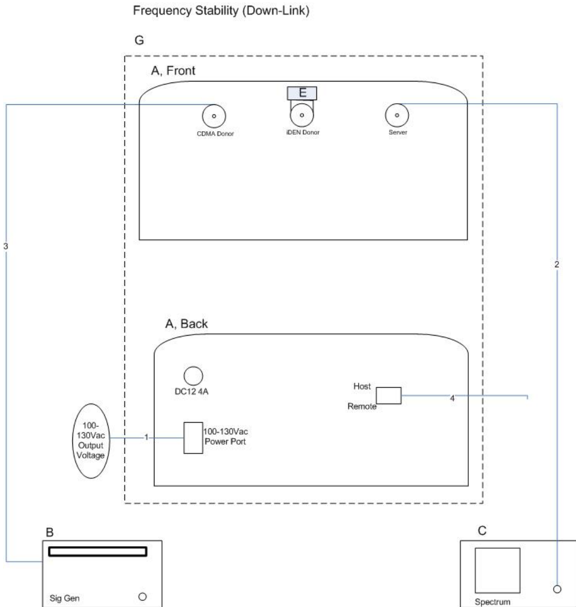
Figure 6. Block Diagram of Test Configuration (Frequency Stability)
