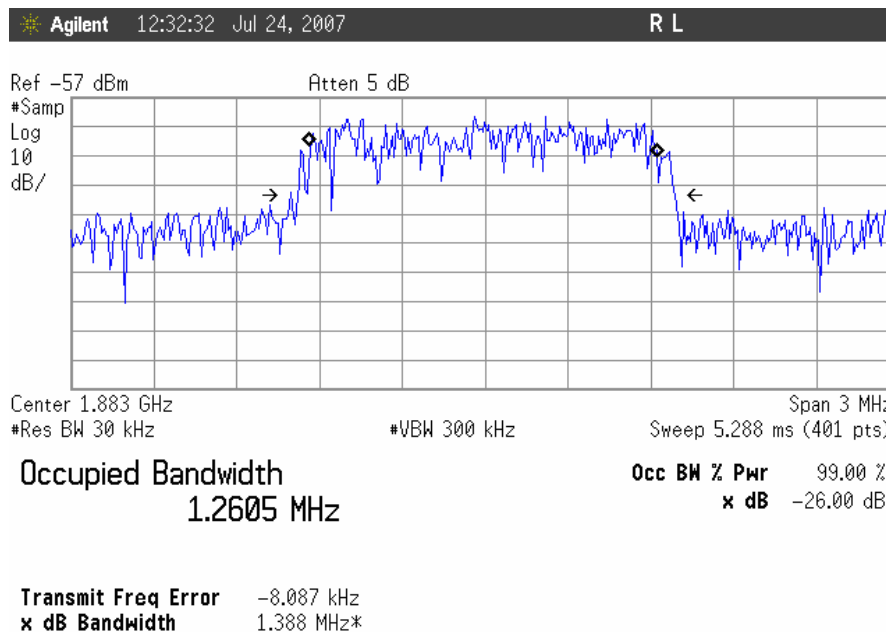
Occupied Bandwidth, CDMA Uplink, Mid Channel Input
