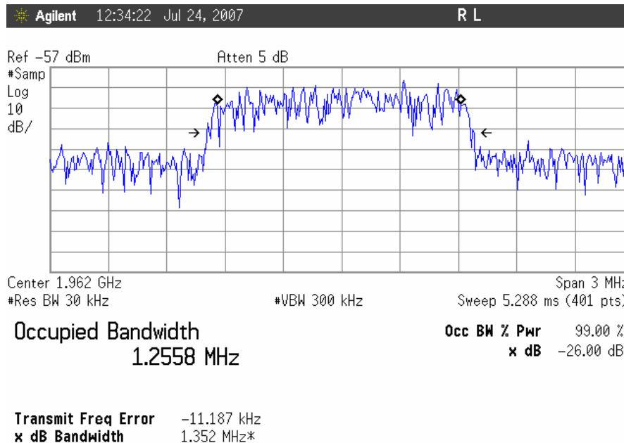
Occupied Bandwidth, CDMA Downlink, Mid Channel Input
