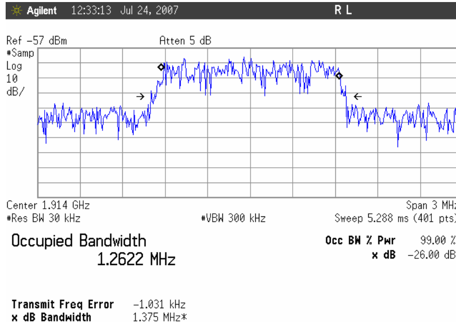
Occupied Bandwidth, CDMA Uplink, High Channel Input
