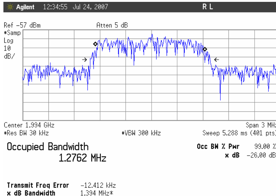
Occupied Bandwidth, CDMA Downlink, High Channel Input
