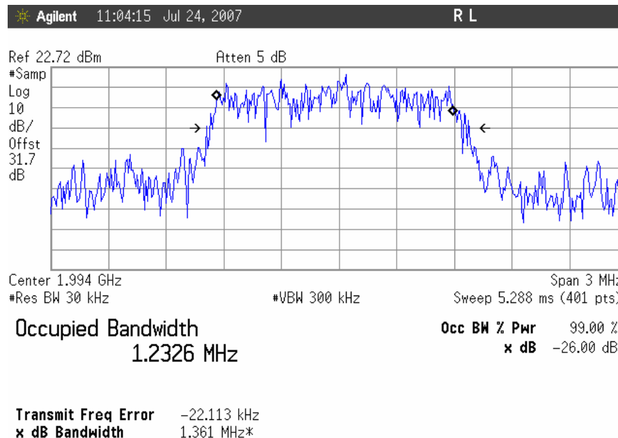
Occupied Bandwidth, CDMA Downlink, High Channel Output
