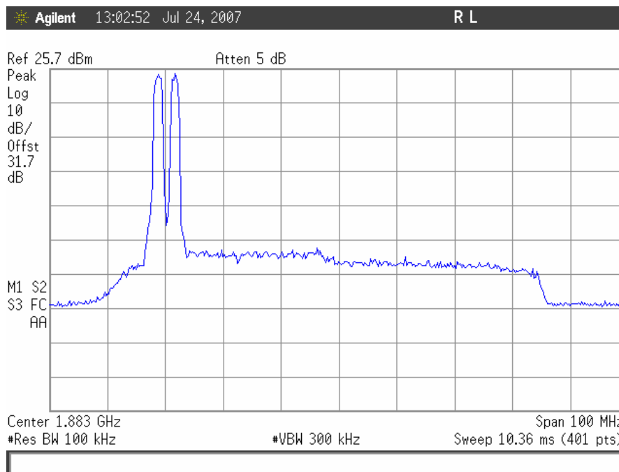
CDMA Intermodulation, Uplink Low End
