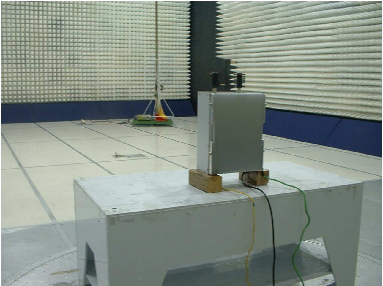
Radiated Emissions at 10 m
