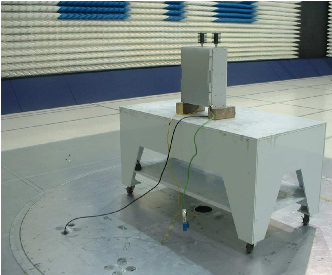
Radiated Emissions at 10 m
