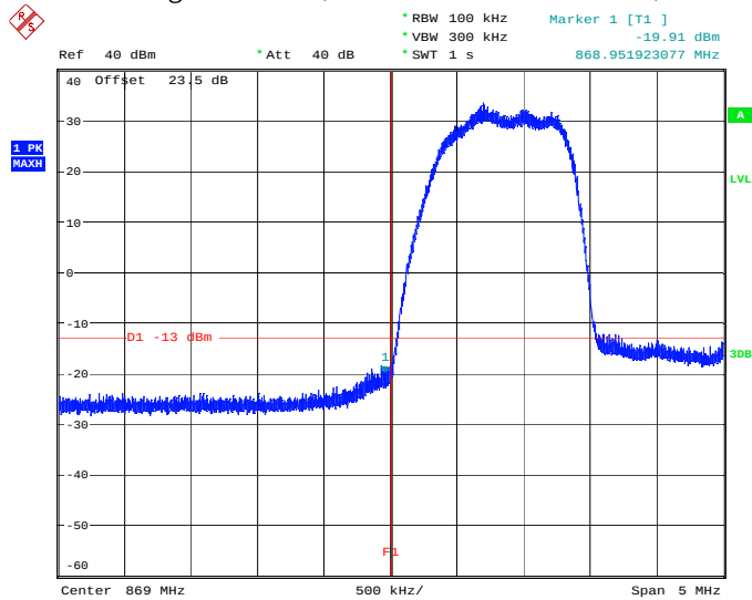
Graph 4.35 Band Edge Emissions, CDMA Cell Channel 1013, Down Link
