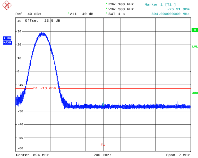
Graph 4.46 Band Edge Emissions, TDMA Cell Channel 777, Down Link
