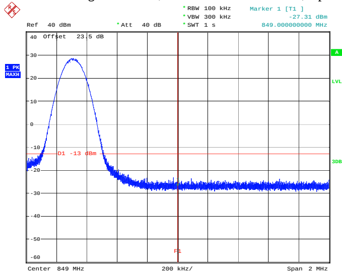
Graph 4.44 Band Edge Emissions, TDMA Cell Channel 777, Up Link
