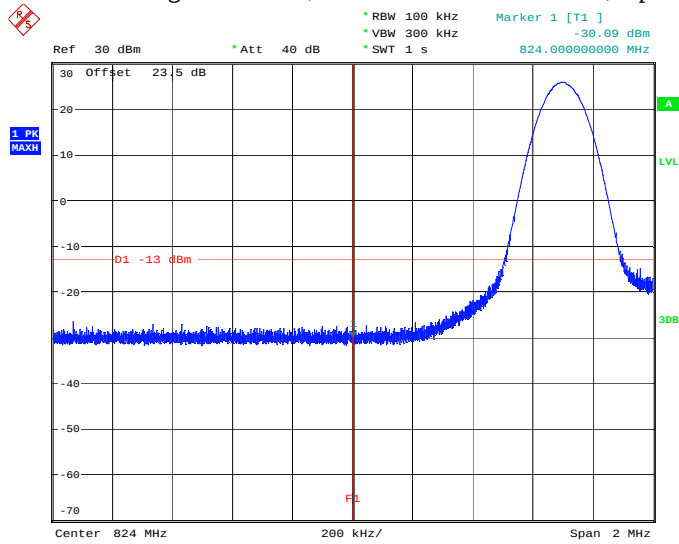
Graph 4.43 Band Edge Emissions, TDMA Cell Channel 1013, Up Link
