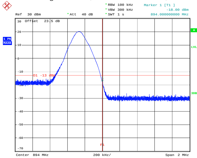
Graph 4.40 Band Edge Emissions, GSM 850 Channel 251, Down Link
