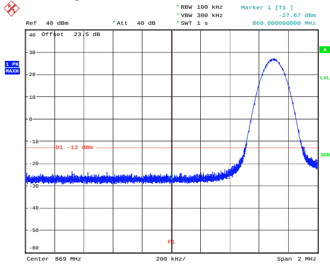
Graph 4.45 Band Edge Emissions, TDMA Cell Channel 1013, Down Link
