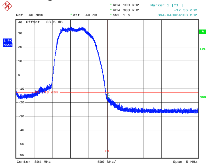
Graph 4.36 Band Edge Emissions, CDMA Cell Channel 777, Down Link
