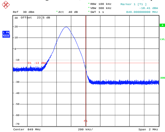
Graph 4.42 Band Edge Emissions, GSM 850 Channel 251, Up Link
