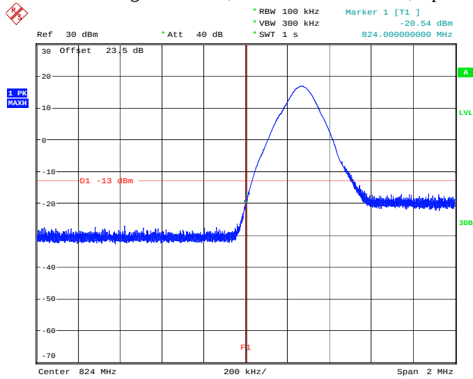
Graph 4.41 Band Edge Emissions, GSM 850 Channel 128, Up Link
