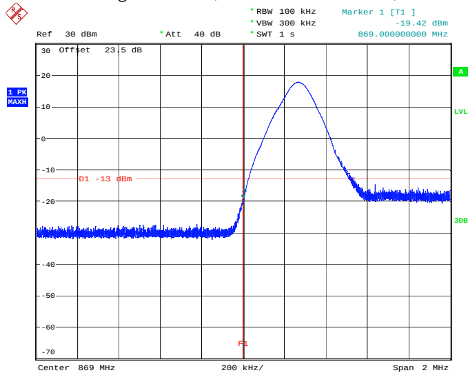
Graph 4.39 Band Edge Emissions, GSM 850 Channel 128, Down Link
