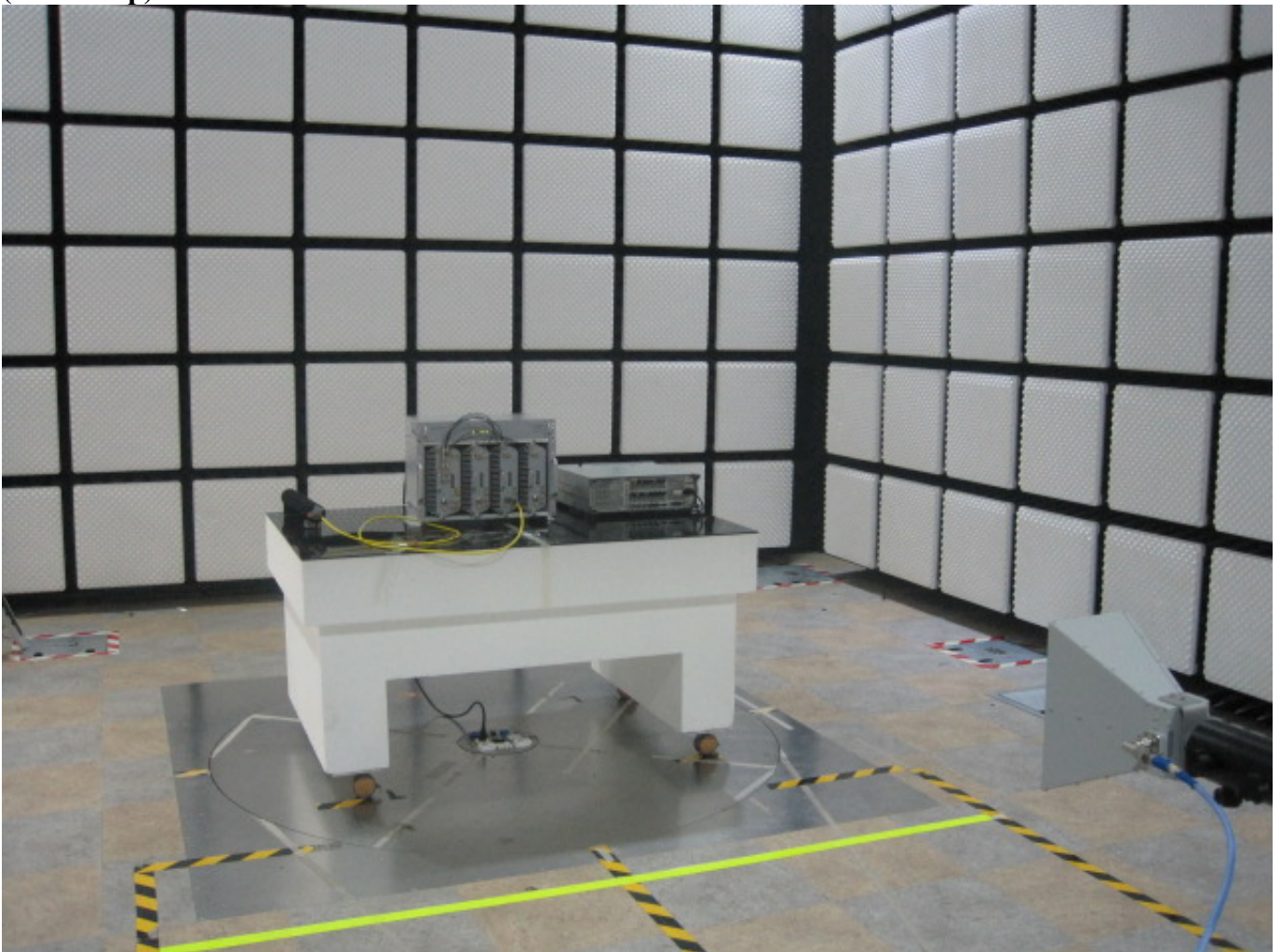
(Test Setup)
