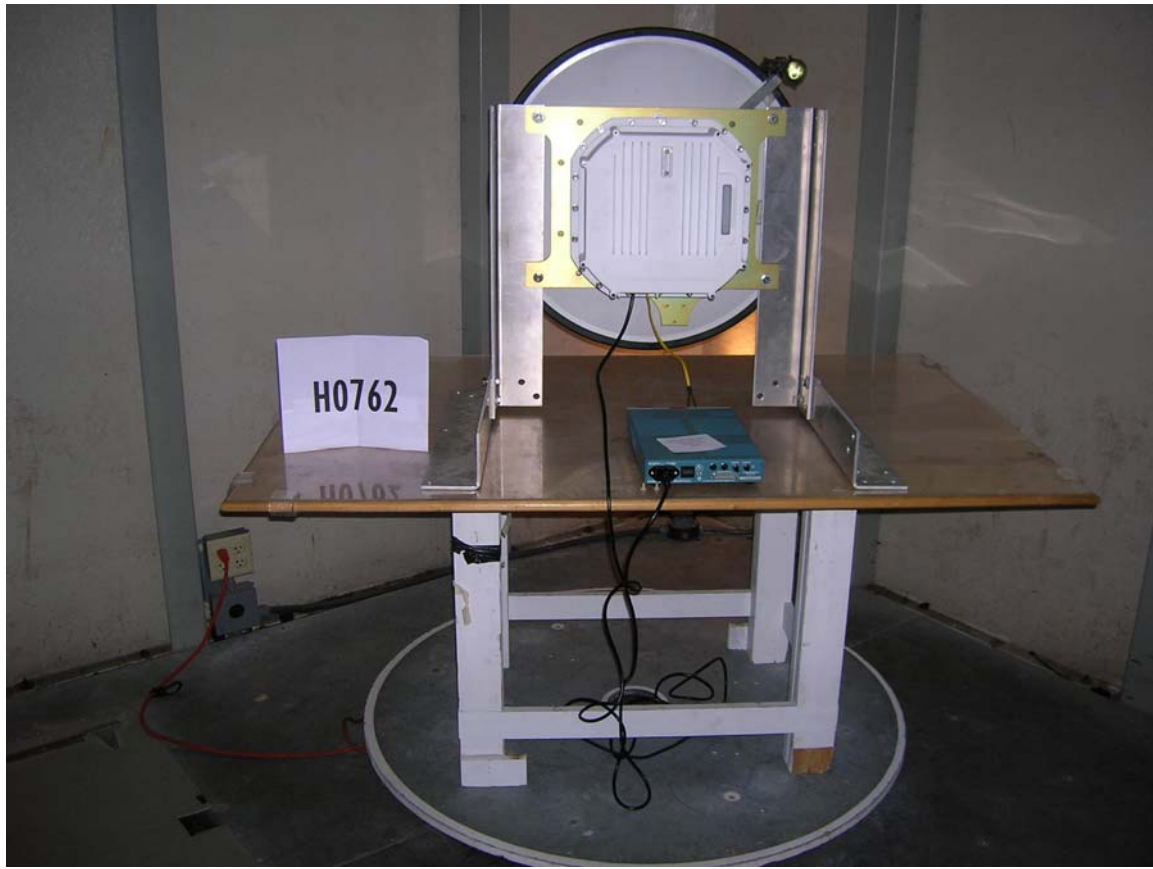
Radiated Spurious Emissions 30-1000MHz – Back
