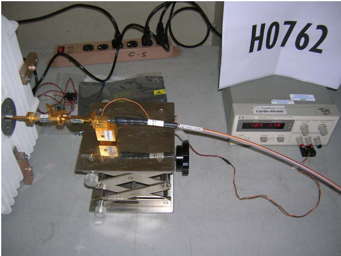
Bandwidth – Block Downconverter
