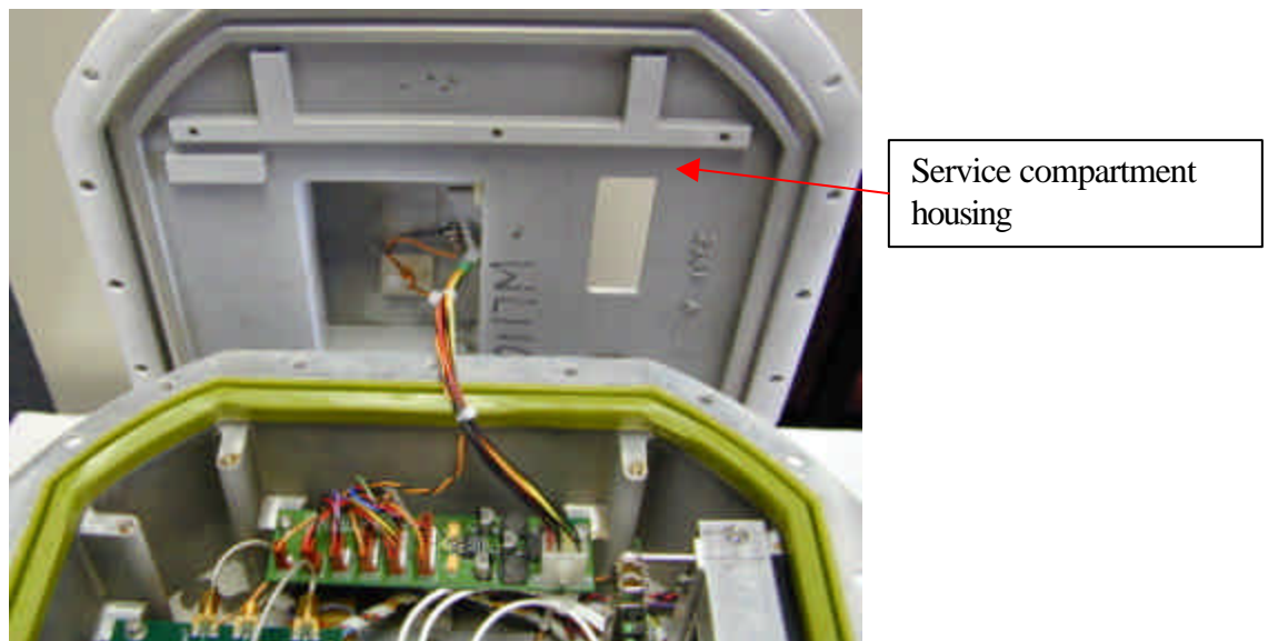
Photo of EUT showing backside of service compartment housing
