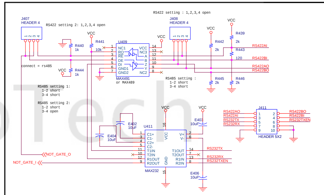
Rs232 to rs422/485 module
