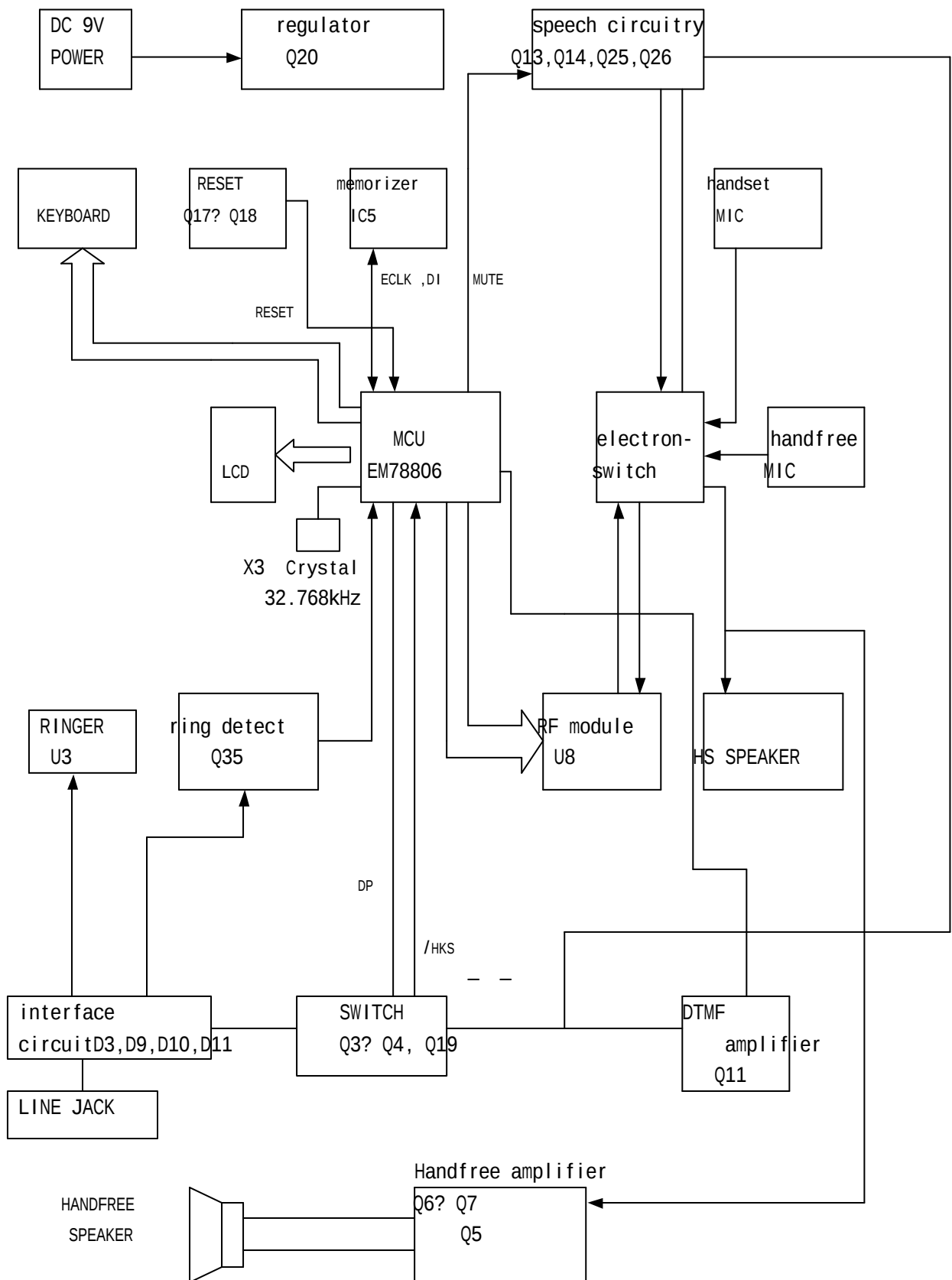
29660 block drawing (base unit)
