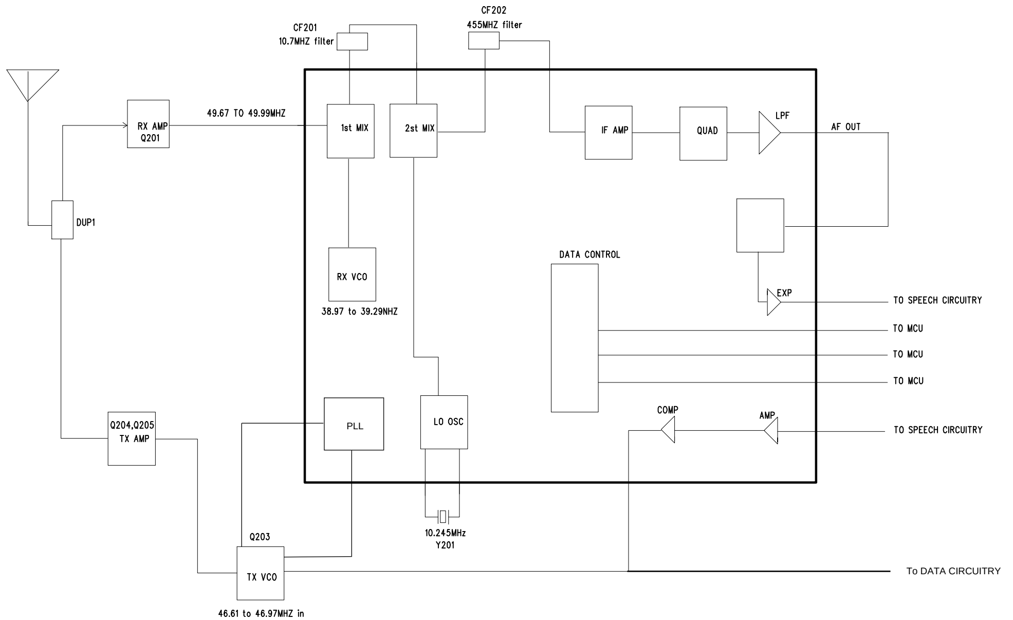
26760/29660 RF Module block drawing(base unit)
