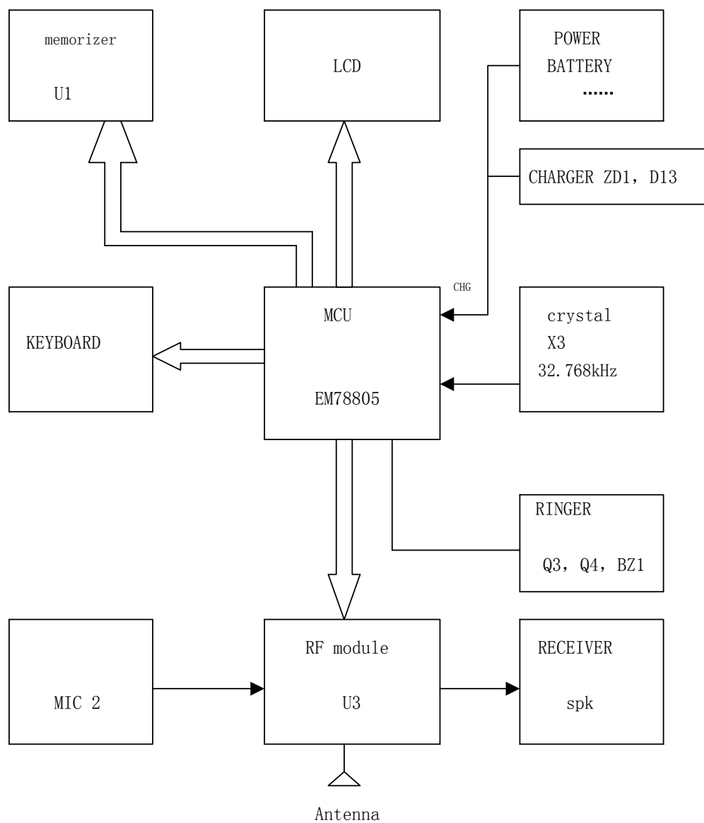
29660/26760 BLOCK DRAWING (HANDSET UNIT)
