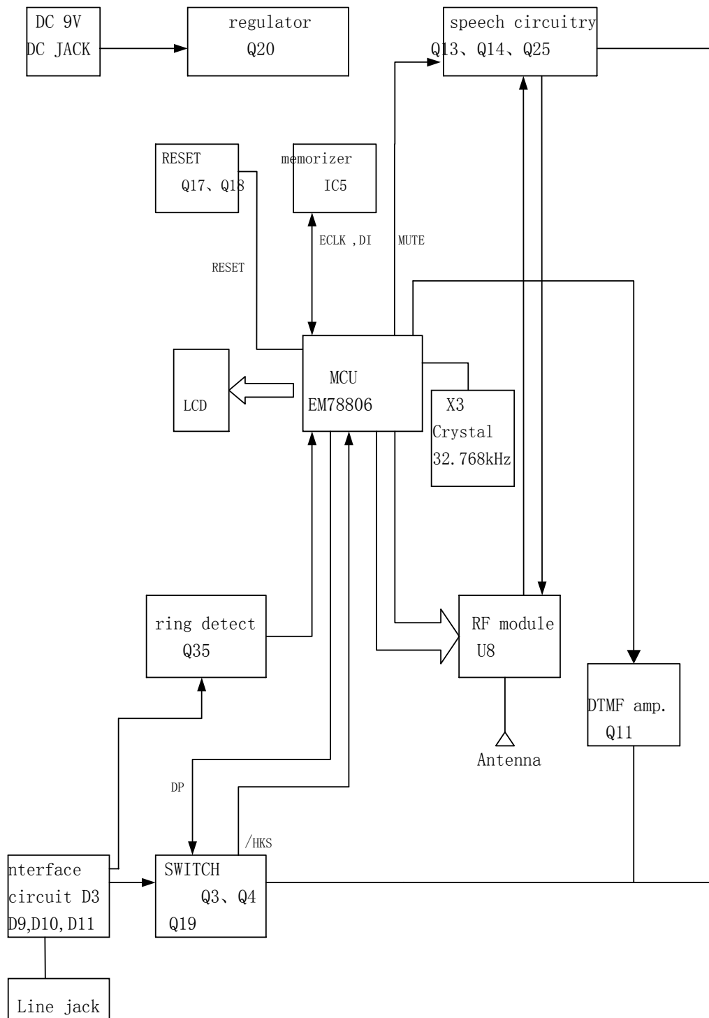
26760 block drawing (base unit)
