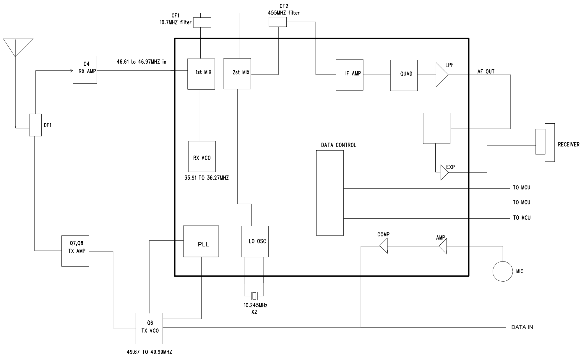
26760/29660 RF Module block drawing(hs unit)
