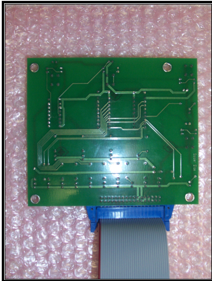
PHOTOGRAPH 40: PC BOARD BACK VIEW
