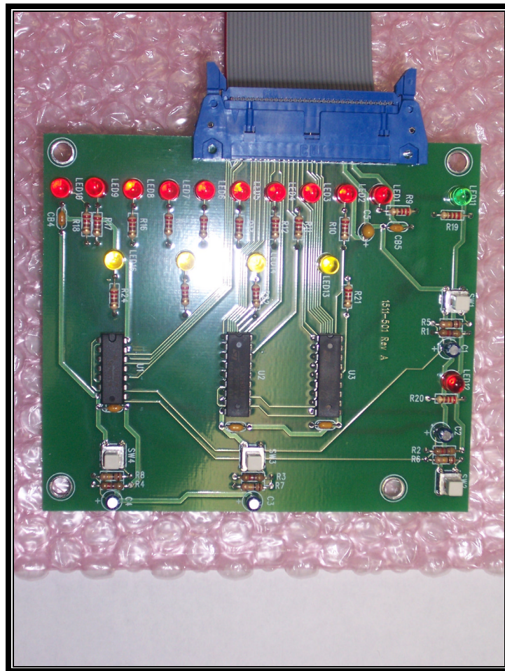
PHOTOGRAPH 39: PC BOARD FRONT VIEW
