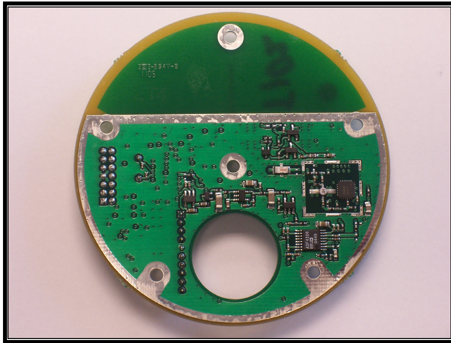
PHOTOGRAPH 38: TX BOARD BACK VIEW
