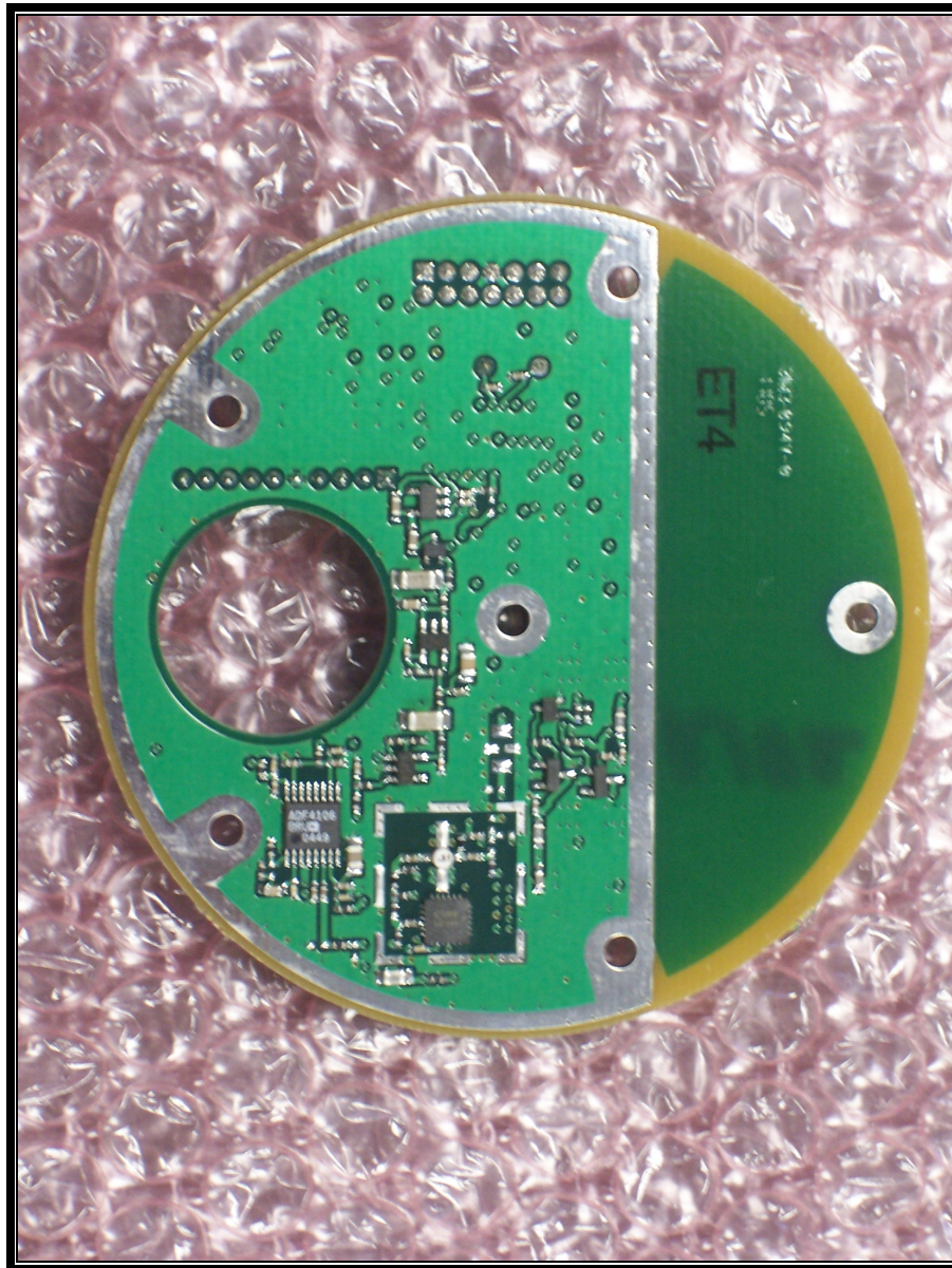
PHOTOGRAPH 31: RX BOARD BACK VIEW
