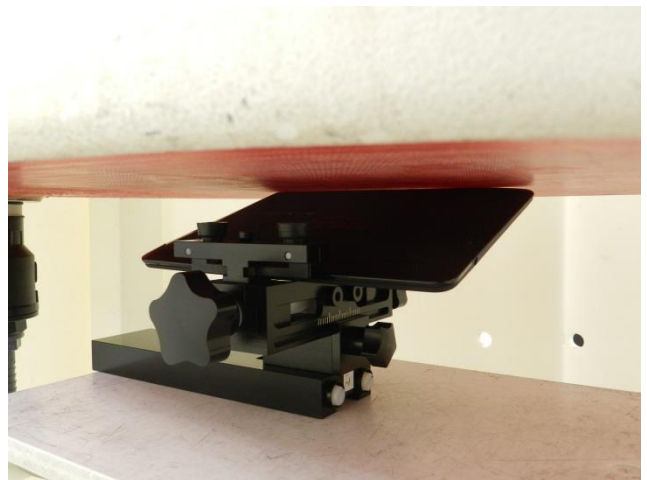
Bottom Face - Slant of Ant 2, Test Separation 0 cm
