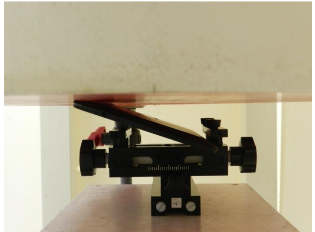
Bottom Face - Slant of Ant 1, Test Separation 0 cm
