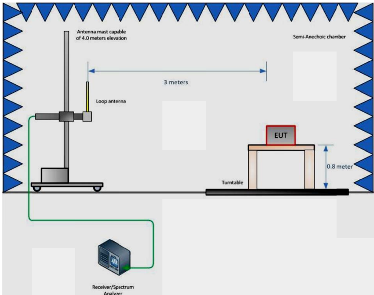
Figure1: Radiated Emission Test Setup (Below 30 MHz)
