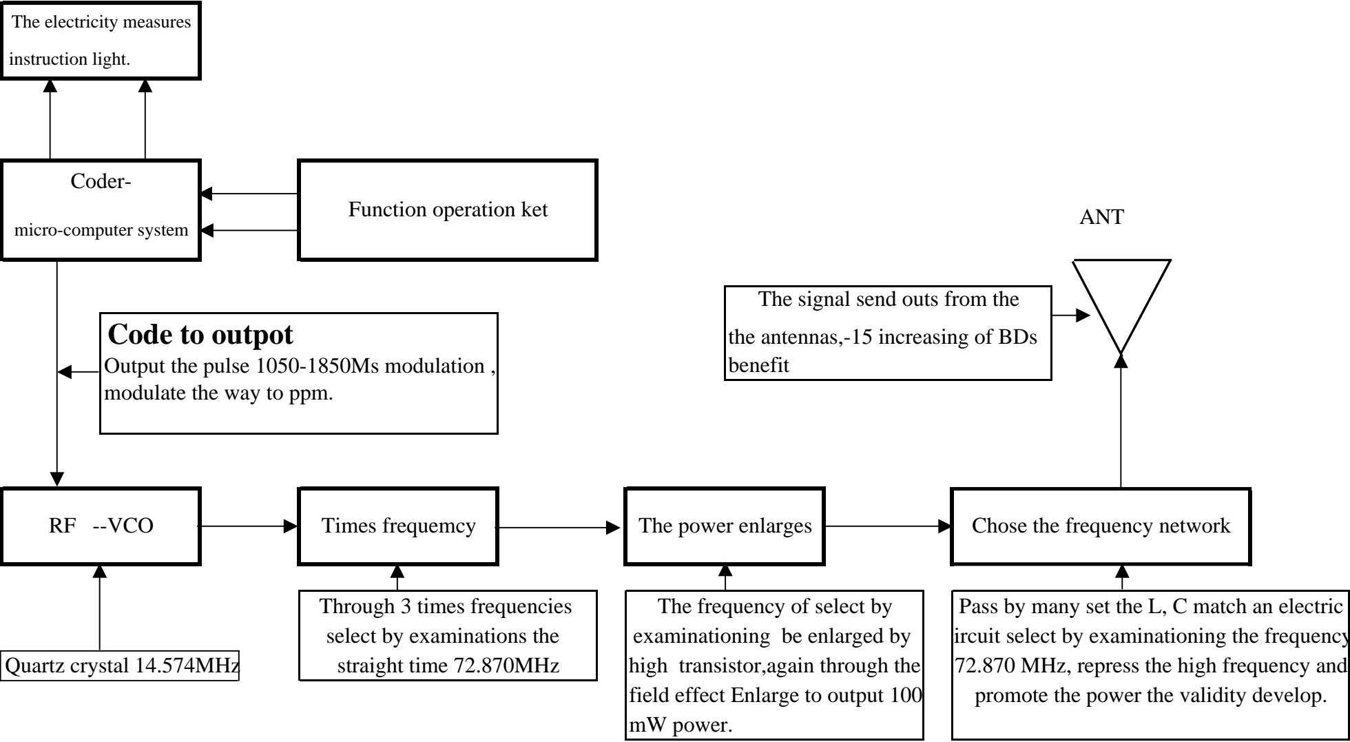
Block Diagram of WK-0405 (72.870MHz)
