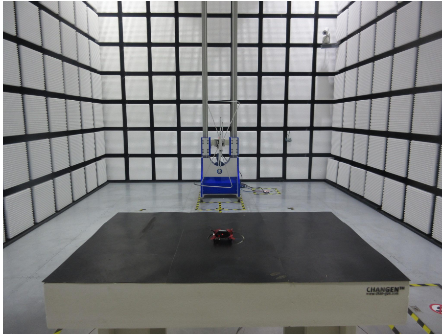
Radiated Emission(30MHz-1GHz)
