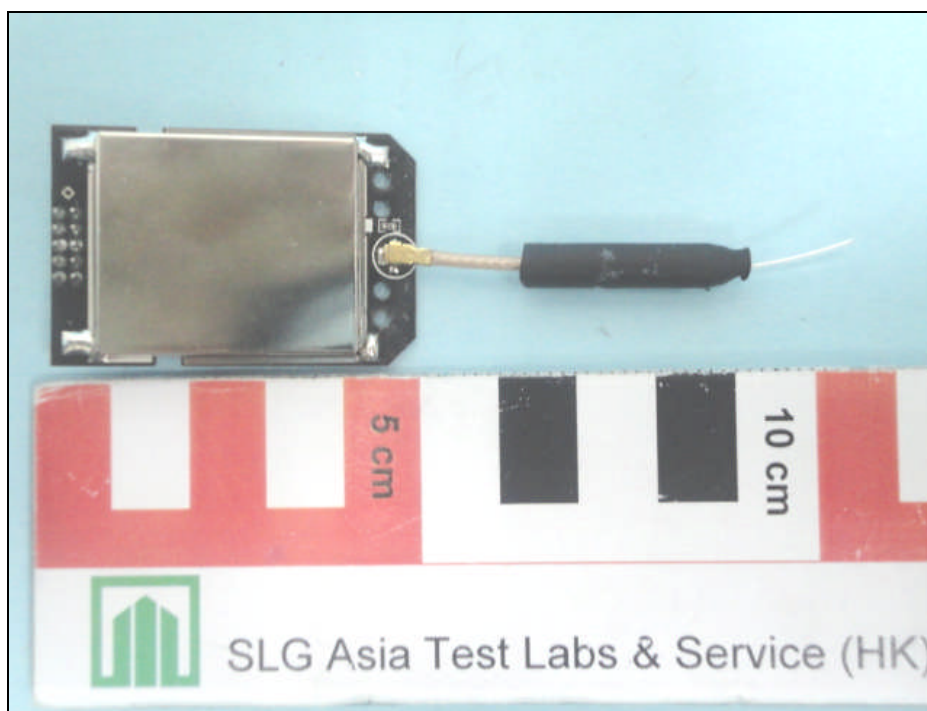
2.4 GHz DSSS Transceiver module with antenna
