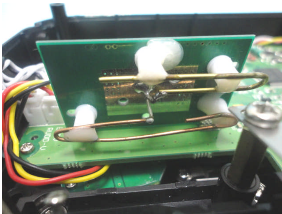
5.8GHz Video receiver antenna
