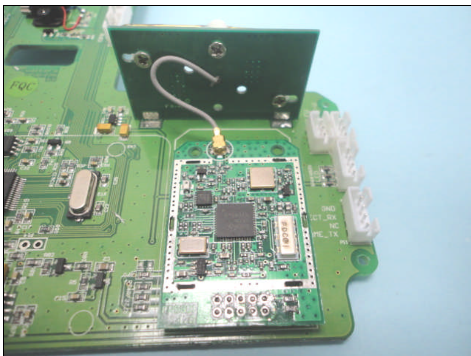
5.8GHz Video receiver module
