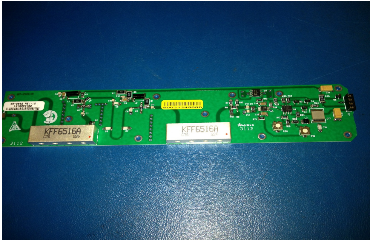
Receiver Board Top
