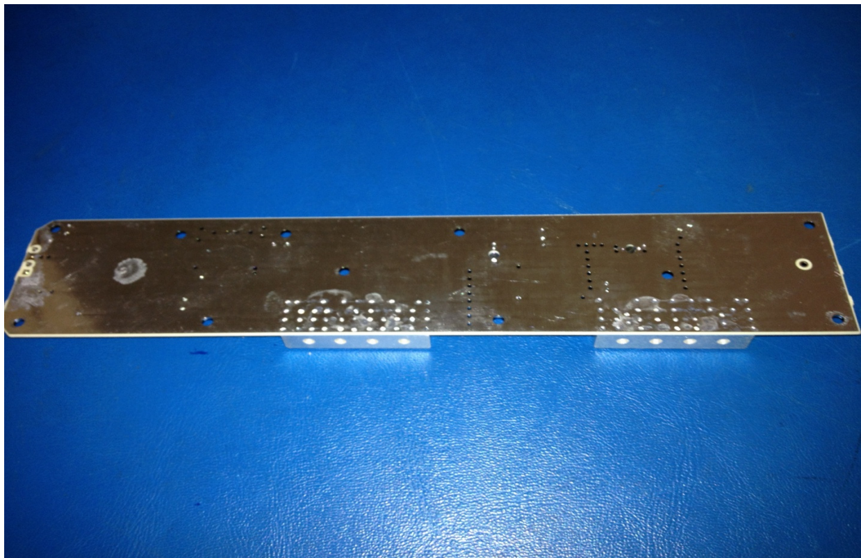
Receiver Board Bottom
