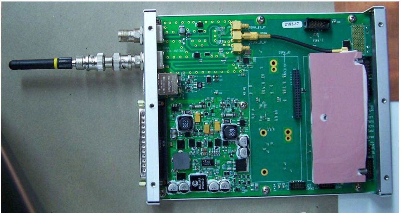
EUT with Cover Removed
