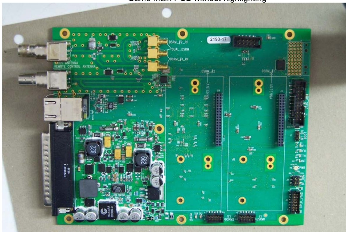
Same Main PCB without highlighting
