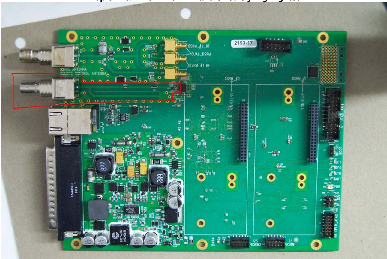
Top of Main PCB with Z-Wave Circuitry highlighted
