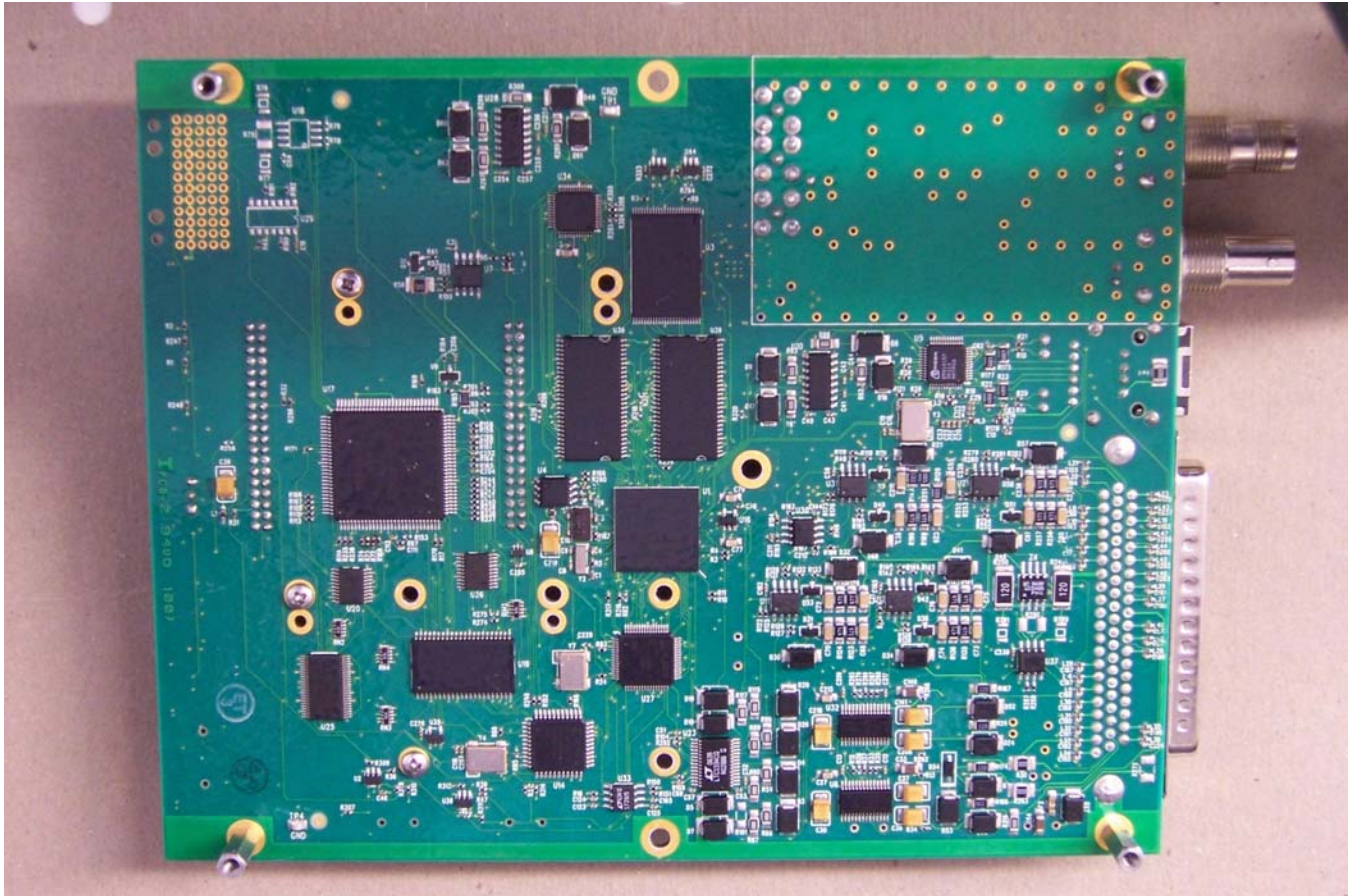
Bottom Side of Main PCB
