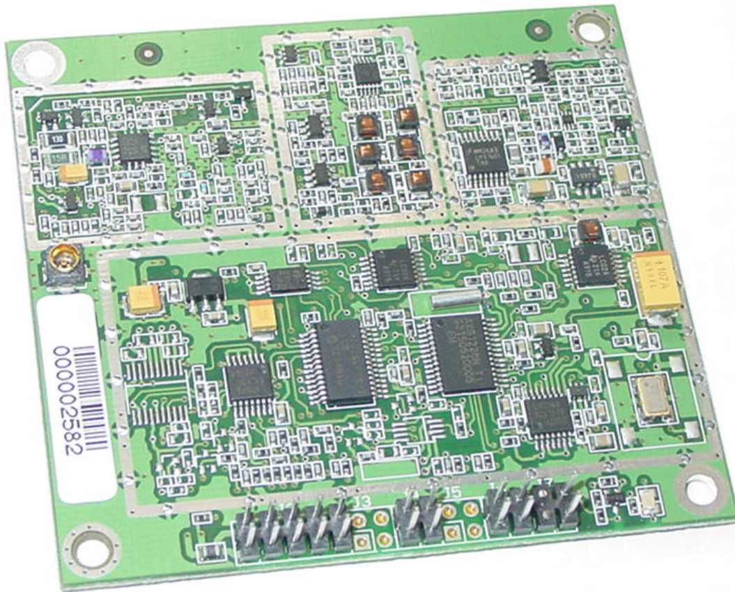
Transmitter board with cover removed
