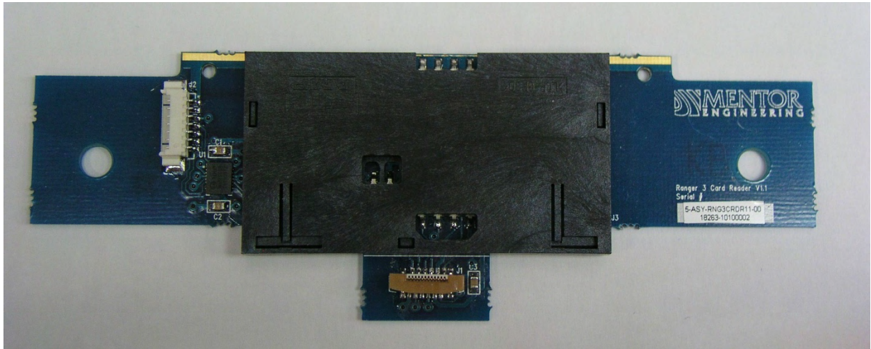
CARD READER BOARD TOP VIEW
