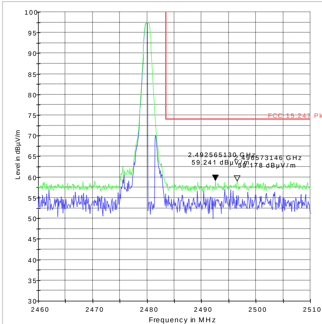
FCC 15.247 HBE Pk 3m
