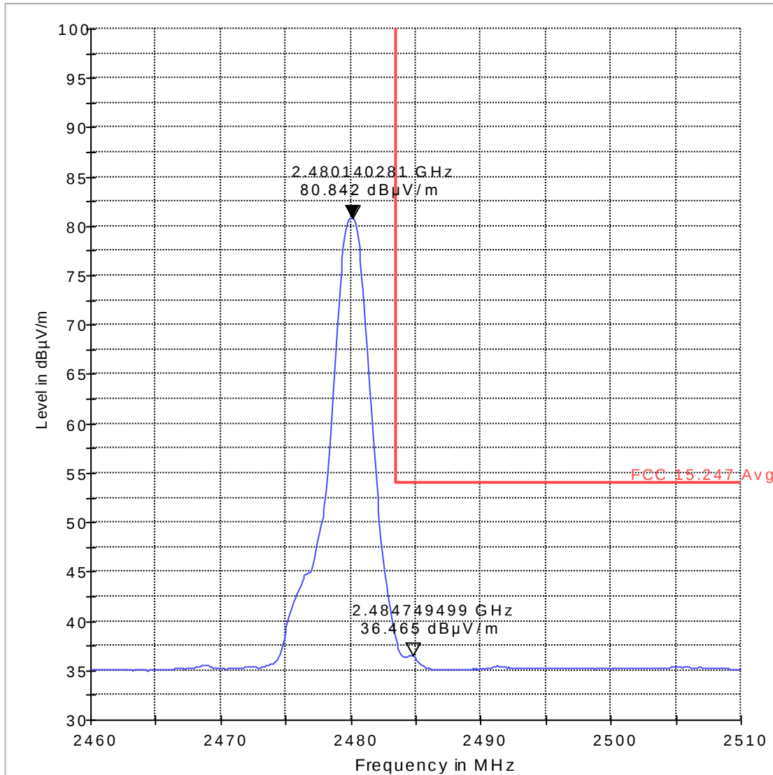
FCC 15.247 HBE Avg 3m
