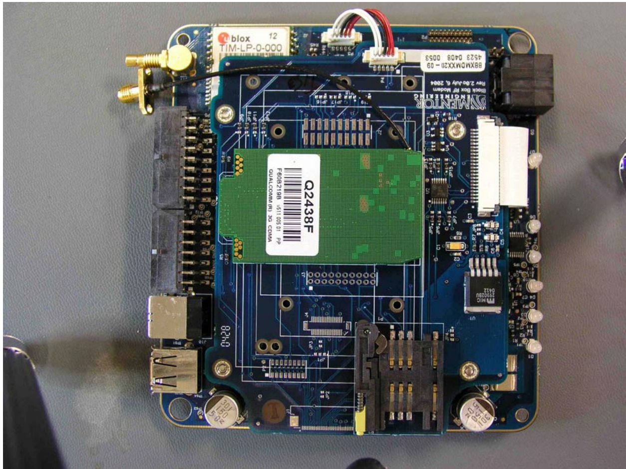
Top Assembly 1
