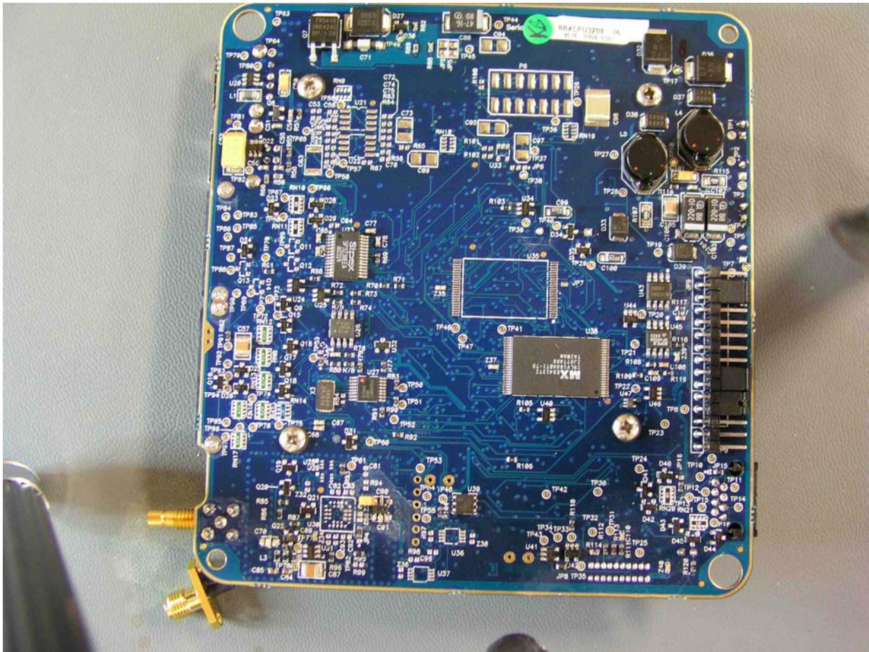
Bottom Assembly 1
