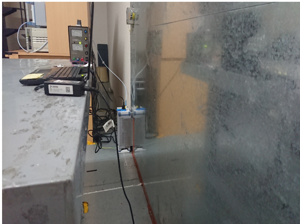
Photograph 8: Set-up for Mains Conducted testing (Back View)
