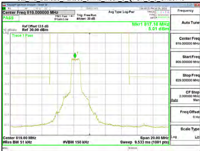
Cat M1 Band26 Part90s 5MHz index 3 QPSK 6 0 CH26765
