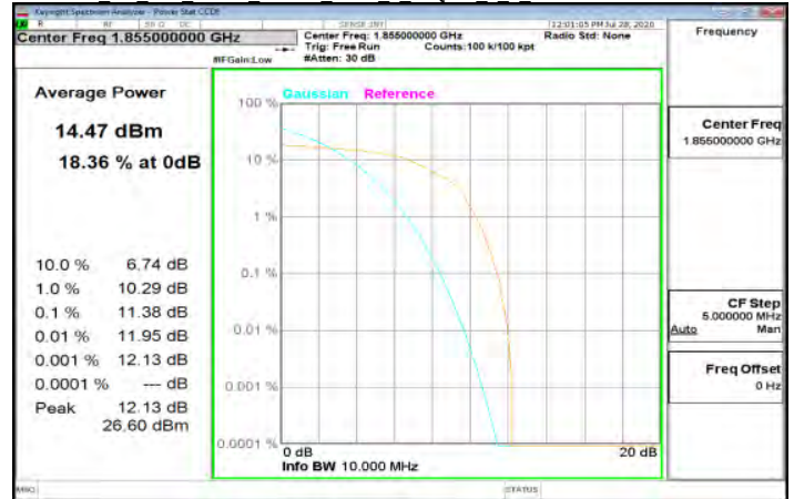
Cat M1 LTE Band2 10MHz index 0 16QAM 6 0 LowCH18650-1855
