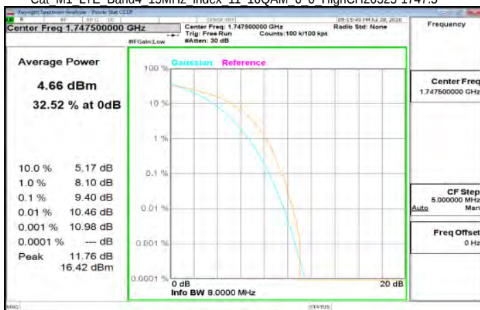
Cat M1 LTE Band4 15MHz index 11 16QAM 6 0 HighCH20325-1747.5
