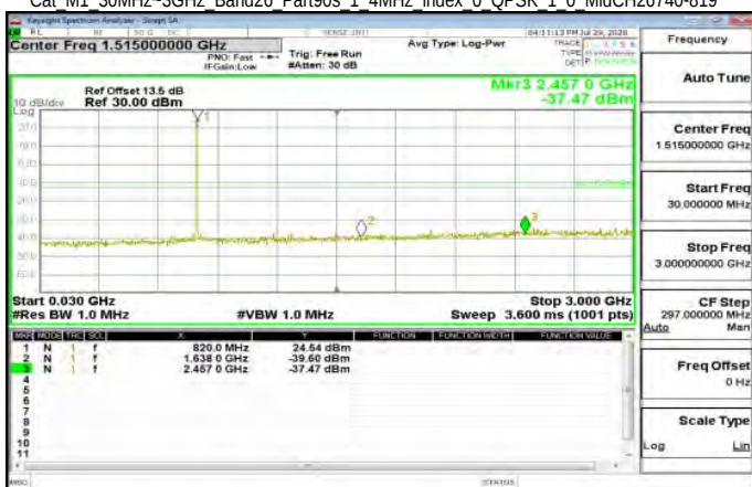
Cat M1 30MHz-3GHz Band26 Part90s 1 4MHz index 0 QPSK 1 0 MidCH26740-819
