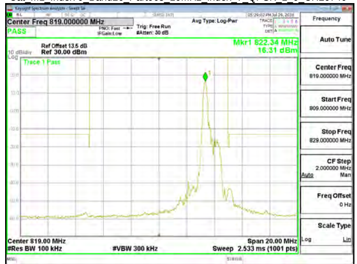
Cat M1 Index 0 Band26 Part90s 10MHz index 0 QPSK 1 5 CH26740
