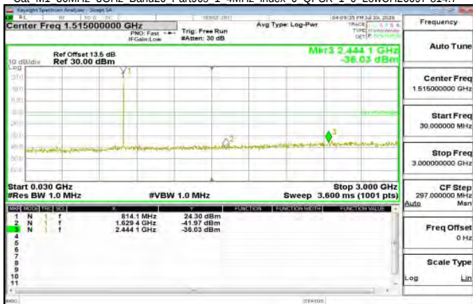
Cat M1 30MHz-3GHz Band26 Part90s 1 4MHz index 0 QPSK 1 0 LowCH26697-814.7
