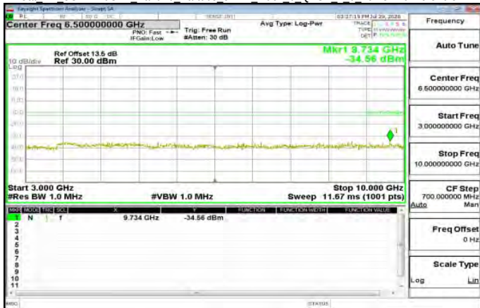
Cat M1 3GHz-10GHz Band26 Part90s 5MHz index 0 QPSK 1 0 LowCH26715-816.5
