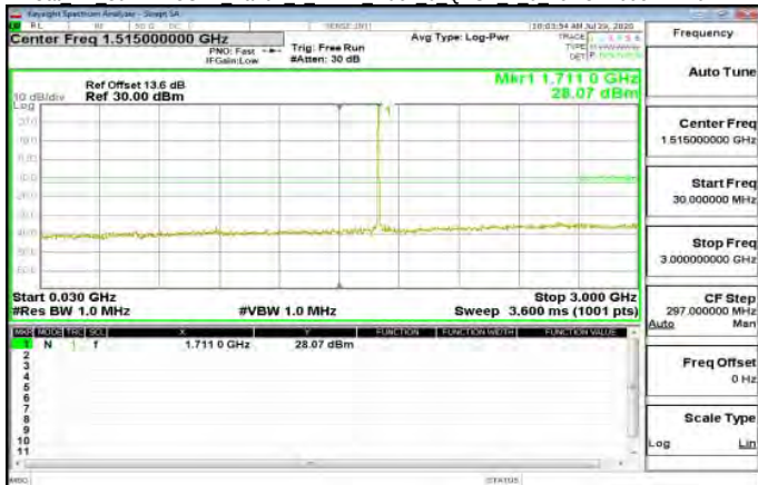
Cat M1 30MHz-3GHz Band4 1 4MHz index 0 QPSK 1 0 LowCH19957-1710.7
