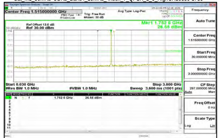
Cat M1 30MHz~3GHz Band4 10MHz index 7 QPSK 1 0 HighCH20350-1750
