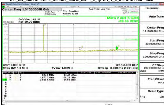
Cat M1 30MHz-3GHz Band26 5MHz index 0 QPSK 1 0 MidCH26915-836.5
