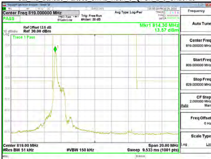
Cat M1 Band26 Part90s 5MHz index 0 QPSK 1 0 CH26740
