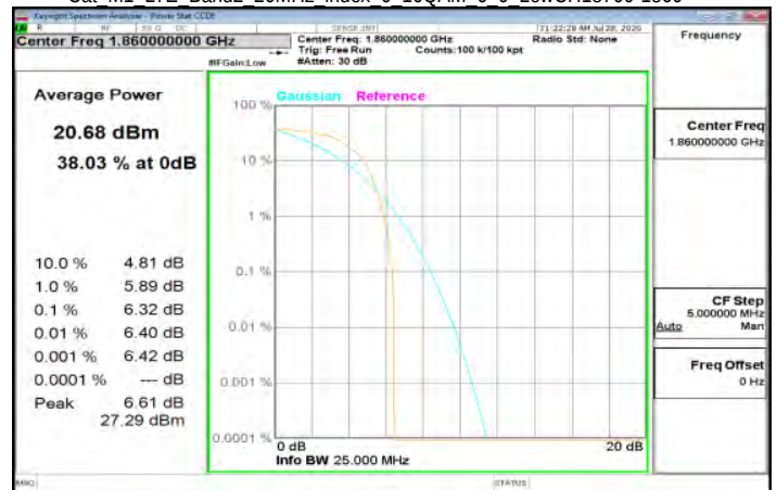
Cat M1 LTE Band2 20MHz index 0 16QAM 6 0 LowCH18700-1860
