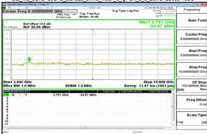
Cat M1 3GHz-10GHz Band12 5MHz index 0 QPSK 1 0 LowCH23035-701.5
