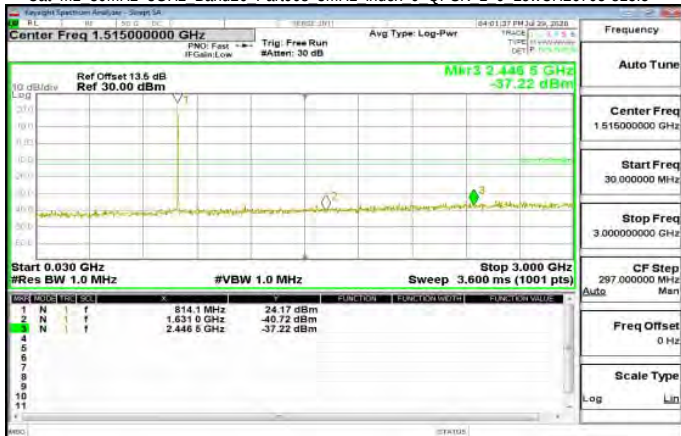
Cat M1 30MHz-3GHz Band26 Part90s 3MHz index 0 QPSK 1 0 LowCH26705-815.5
