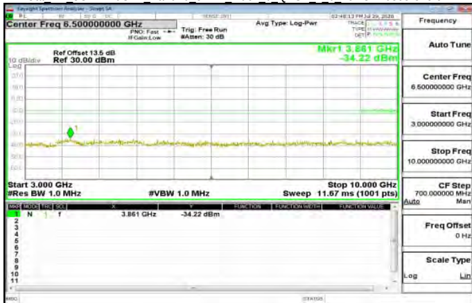
Cat M1 3GHz-10GHz Band26 3MHz index 0 QPSK 1 0 LowCH26805-825.5
