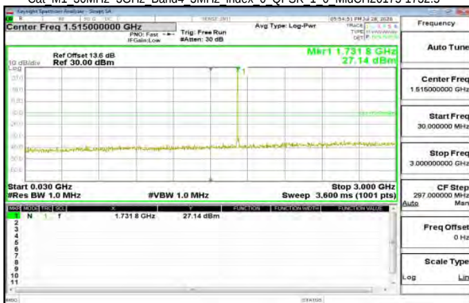
Cat M1 30MHz-3GHz Band4 3MHz index 0 QPSK 1 0 MidCH20175-1732.5
