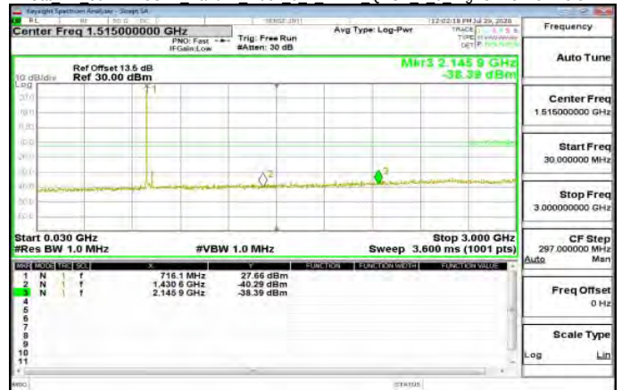
Cat M1 30MHz-3GHz Band12 index 0 1 4MHz QPSK 1 0 HighCH23173-715.3
