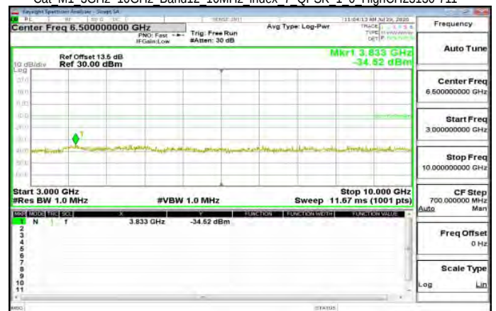
Cat M1 3GHz~10GHz Band12 10MHz index 7 QPSK 1 0 HighCH23130-711
