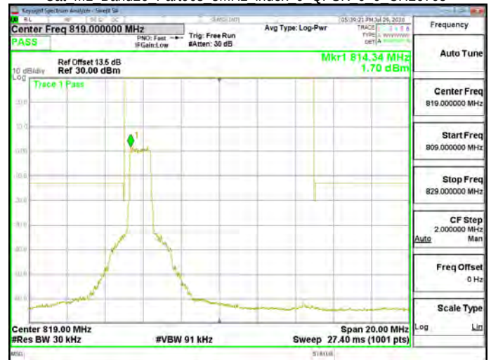
Cat M1 Band26 Part90s 3MHz index 0 QPSK 6 0 CH26740
