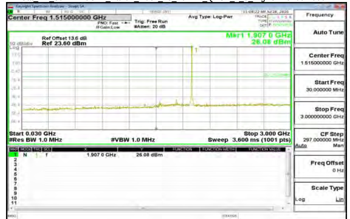
Cat M1 30MHz~3GHz Band2 index 15 20MHz QPSK 1 0 HighCH19100-1900
