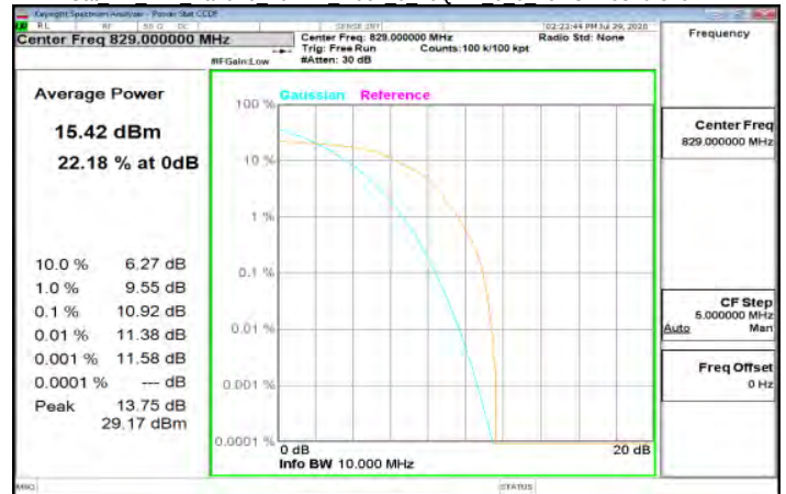
Cat M1 LTE Band26 10MHz index 0 16QAM 6 0 LowCH26840-829
