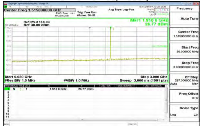
Cat M1 30MHz-3GHz Band2 5MHz index 3 QPSK 1 0 HighCH19175-1907.5
