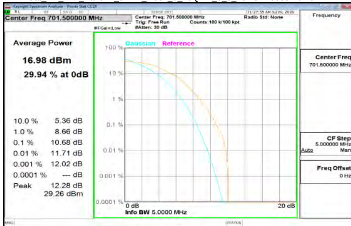
Cat M1 LTE Band12 5MHz index 0 16QAM 6 0 LowCH23035-701.5
