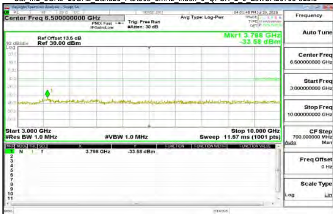
Cat M1 3GHz-10GHz Band26 Part90s 3MHz index 0 QPSK 1 0 LowCH26705-815.5
