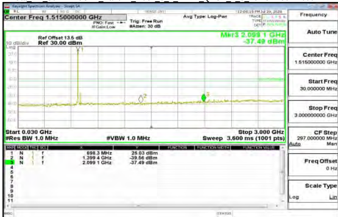
Cat M1 30MHz-3GHz Band12 index 0 1 4MHz QPSK 1 0 LowCH23017-699.7
