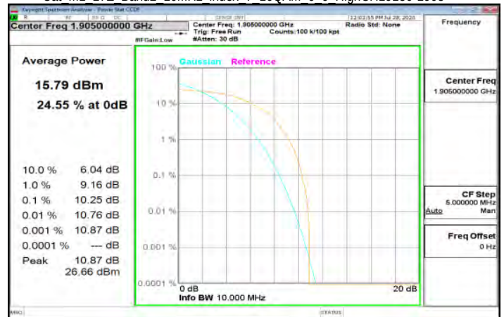
Cat M1 LTE Band2 10MHz index 7 16QAM 6 0 HighCH19150-1905
