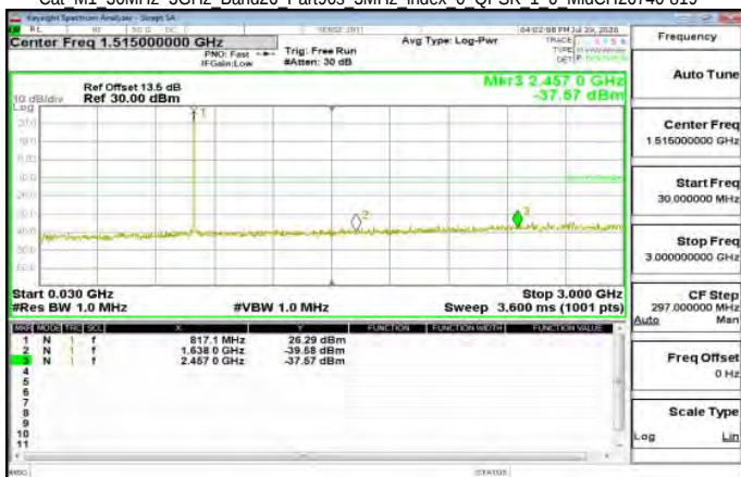
Cat M1 30MHz-3GHz Band26 Part90s 3MHz index 0 QPSK 1 0 MidCH26740-819
