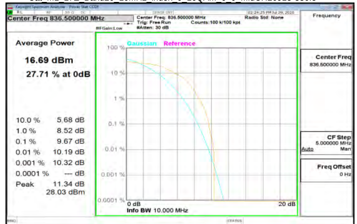
Cat M1 LTE Band26 10MHz index 0 16QAM 6 0 MidCH26915-836.5
