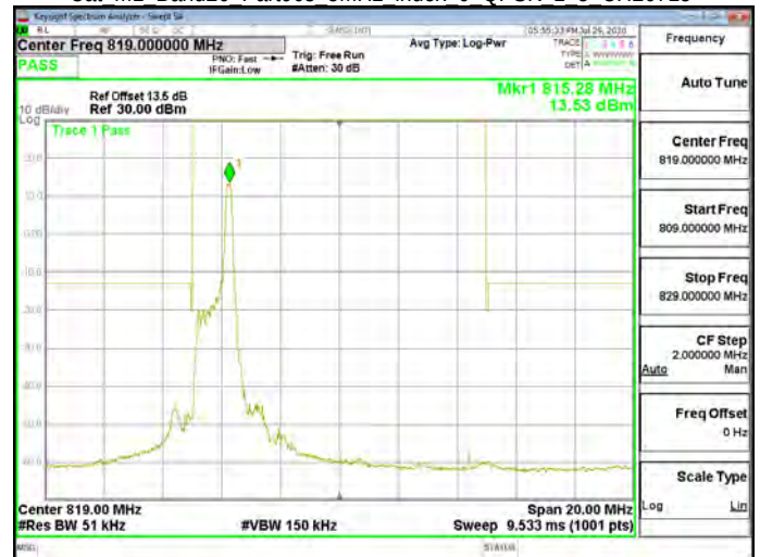
Cat M1 Band26 Part90s 5MHz index 0 QPSK 1 5 CH26740
