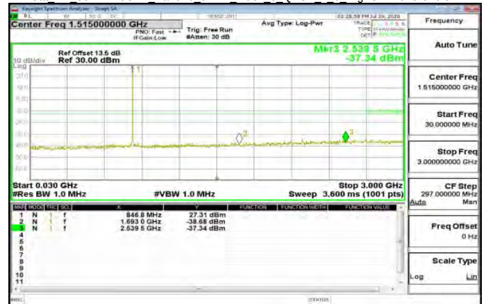
Cat M1 30MHz-3GHz Band26 5MHz index 3 QPSK 1 0 HighCH27015-846.5
