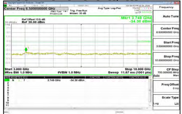
Cat M1 3GHz-10GHz Band26 Part90s 5MHz index 0 QPSK 1 0 MidCH26740-819
