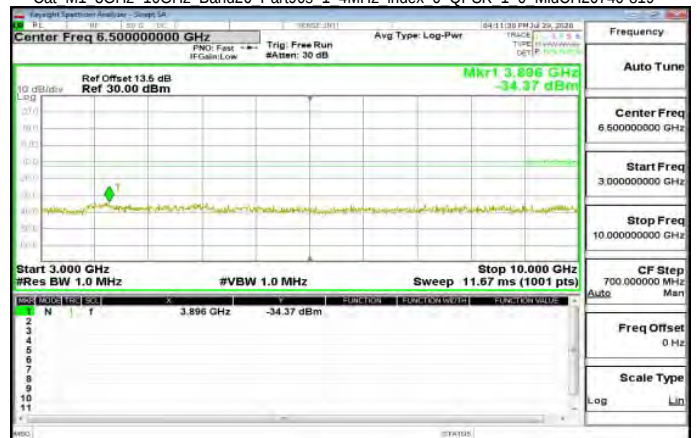
Cat M1 3GHz-10GHz Band26 Part90s 1 4MHz index 0 QPSK 1 0 MidCH26740-819
