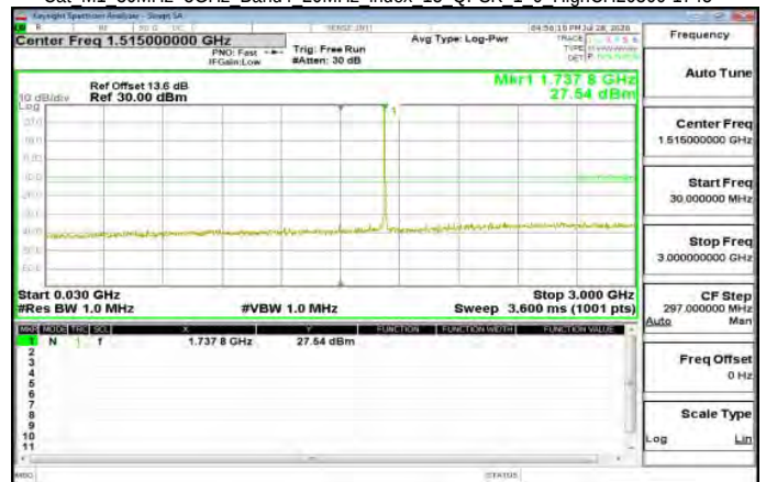
Cat M1 30MHz~3GHz Band4 20MHz index 15 QPSK 1 0 HighCH20300-1745
