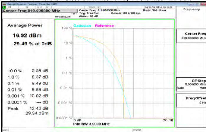
Cat M1 LTE Band26 Part90s 3MHz index 0 16QAM 6 0 MidCH26740-819
