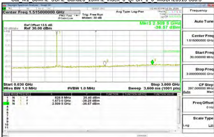
Cat M1 30MHz~3GHz Band26 15MHz index 0 QPSK 1 0 MidCH26915-836.5
