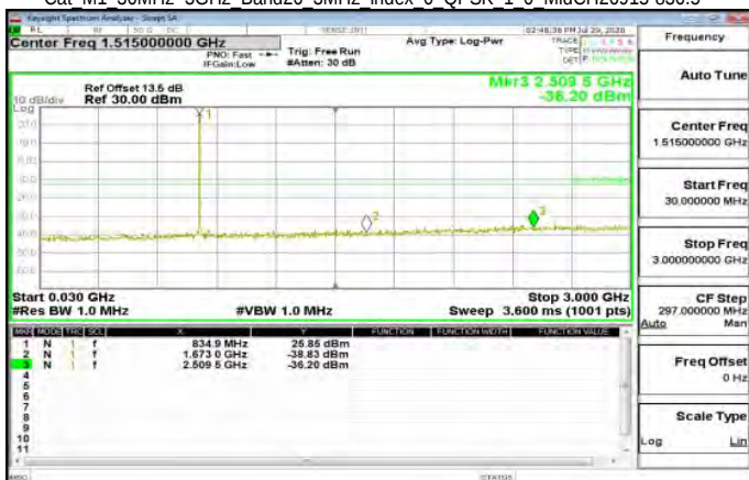
Cat M1 30MHz-3GHz Band26 3MHz index 0 QPSK 1 0 MidCH26915-836.5
