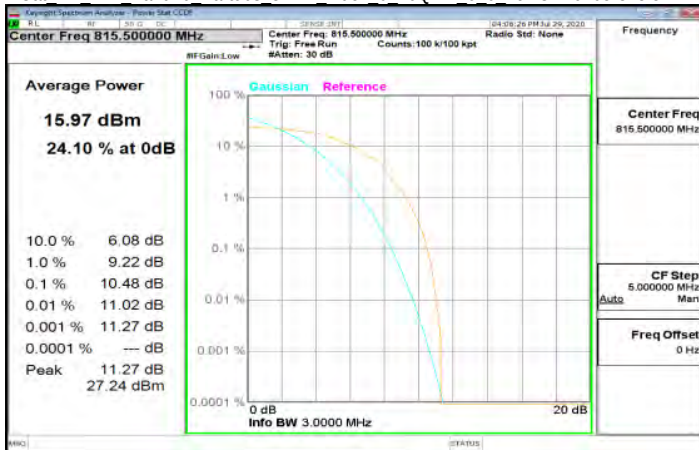
Cat M1 LTE Band26 Part90s 3MHz index 0 16QAM 6 0 LowCH26705-815.5
