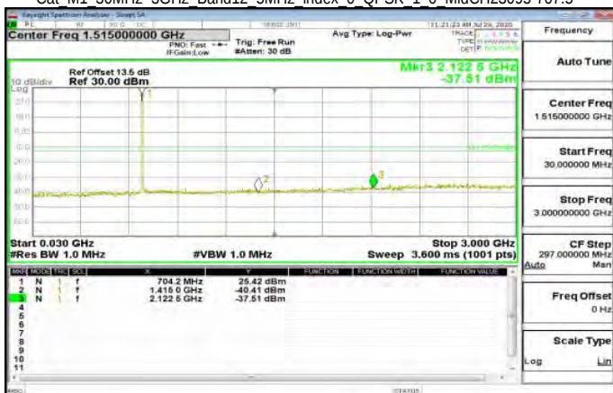
Cat M1 30MHz-3GHz Band12 5MHz index 0 QPSK 1 0 MidCH23095-707.5
