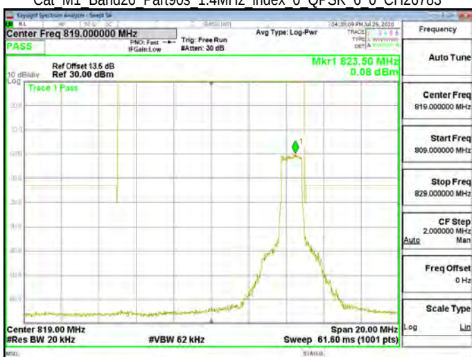
Cat M1 Band26 Part90s 1.4MHz index 0 QPSK 6 0 CH26783
