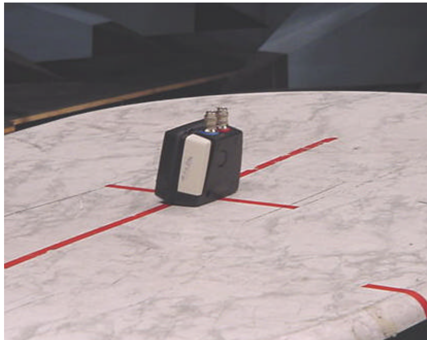
Measurement unit, radiated spurious emission 30 - 1000 MHz
