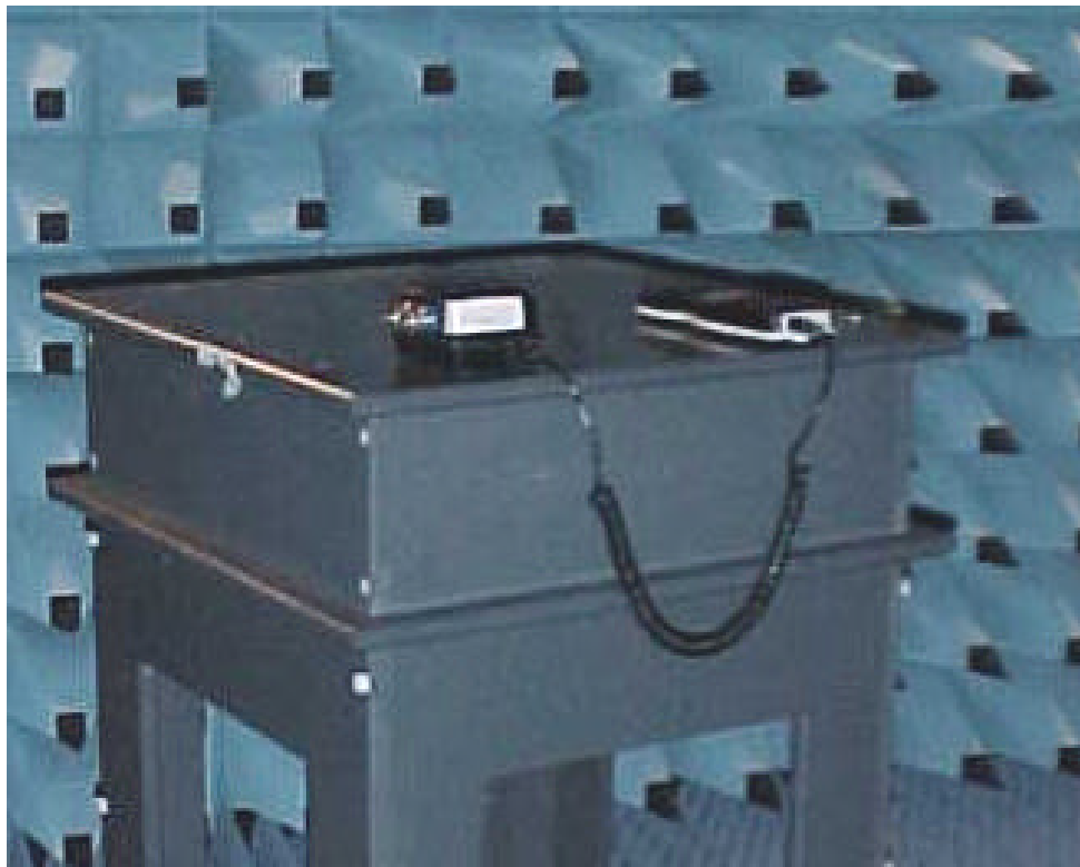
Test set-up stand by mode, 1 – 26 GHz
