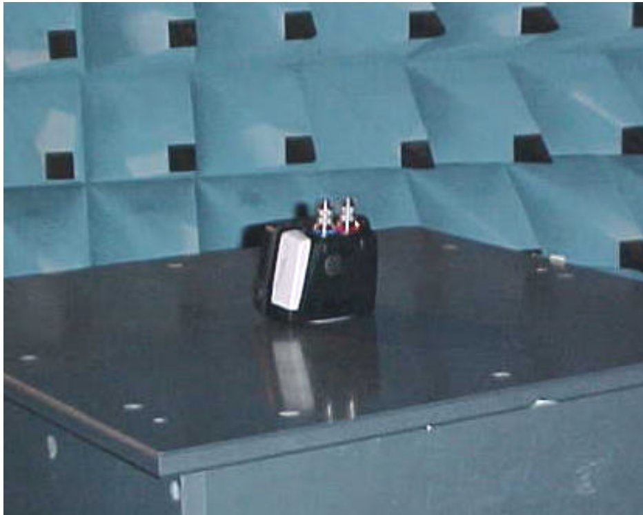
Measurement unit, radiated spurious emission 1 – 26 GHz
