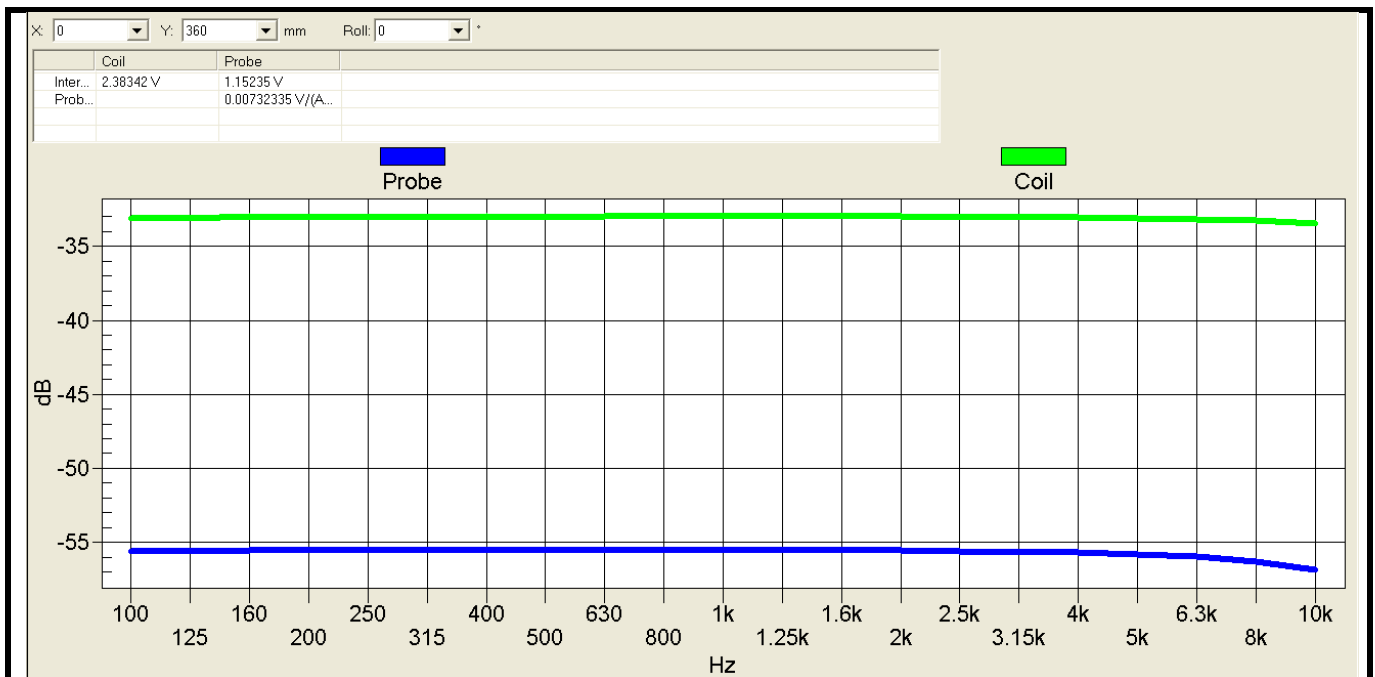
Fig-3.4 Frequency Response and Sensitivity of AM1D Probe
