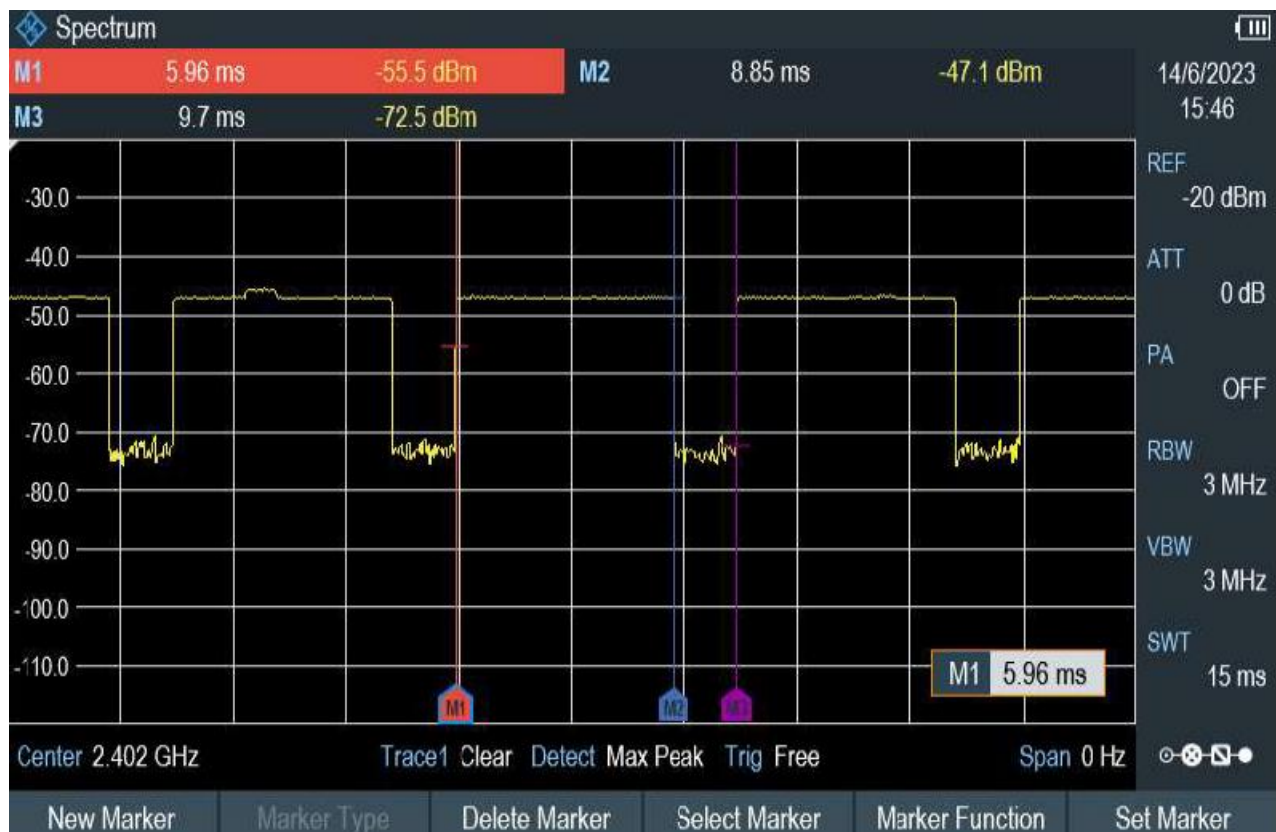
Time-domain plot for Bluetooth transmission signal
