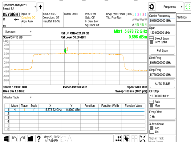
802.11ax_80MHz_Chain3_5690MHz_UNII 3
