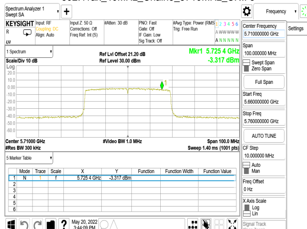
802.11ax_40MHz_Chain3_5710MHz_UNII 3
