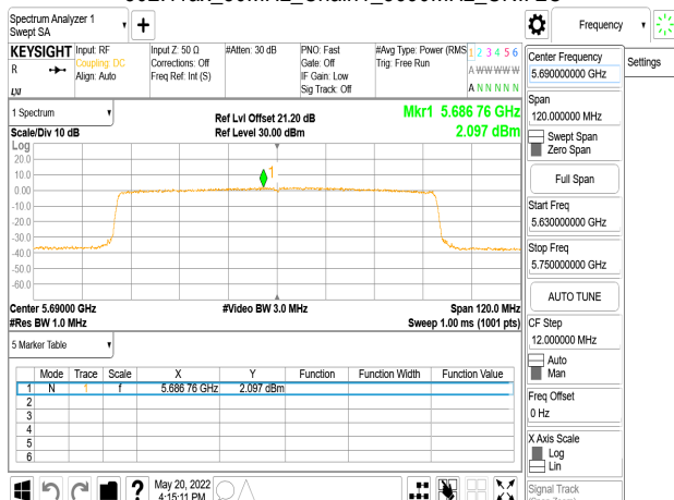
802.11ax_80MHz_Chain1_5690MHz_UNII 2C
