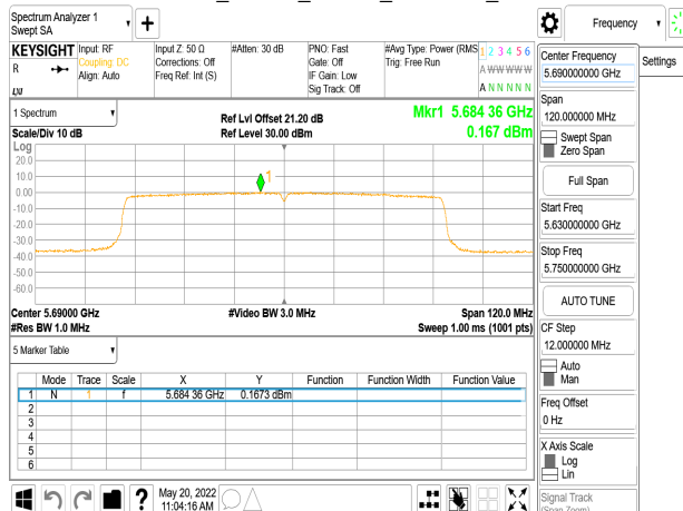
802.11ac_80MHz_Chain0_5690MHz_UNII 2C
