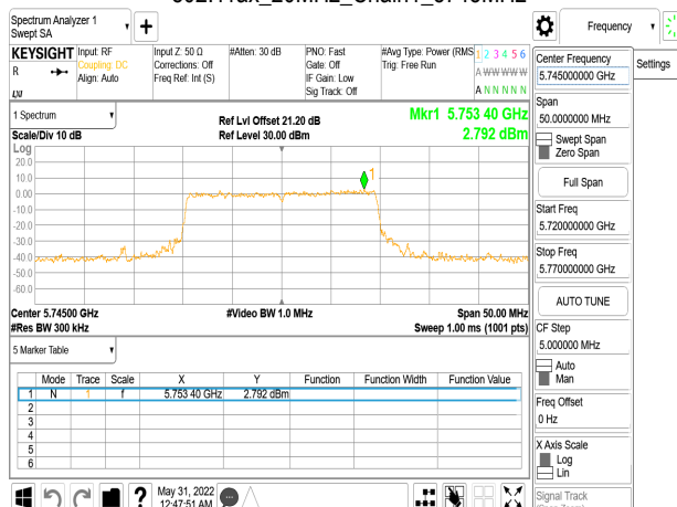
802.11ax_20MHz_Chain1_5745MHz_RU106_53
