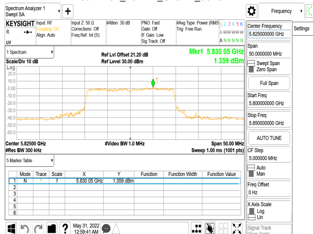
802.11ax_20MHz_Chain1_5825MHz_RU106_54
