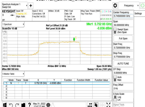
802.11ax_20MHz_Chain0_5745MHz_RU106_53
