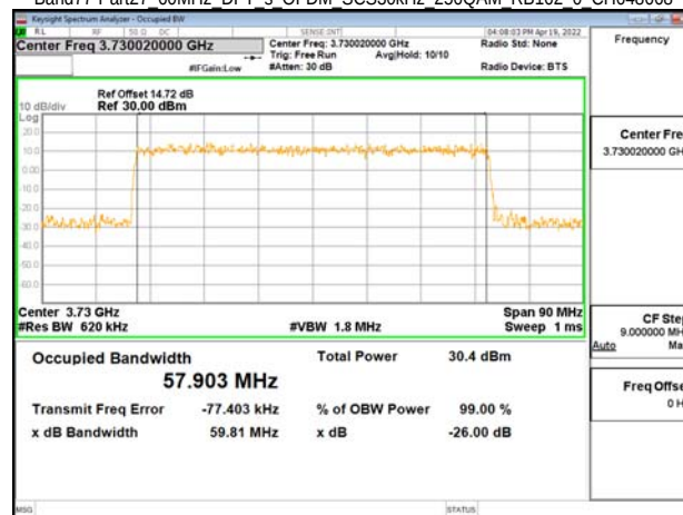
Band77-Part27 60MHz DFT s OFDM SCS30kHz 256QAM RB162 0 CH648668
