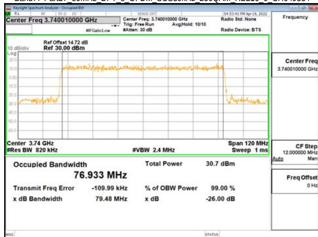
Band77-Part27 80MHz DFT s OFDM SCS30kHz 256QAM RB216 0 CH649334
