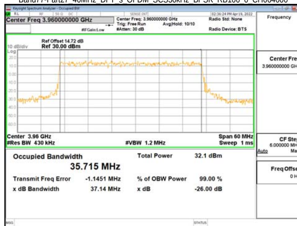
Band77-Part27 40MHz DFT s OFDM SCS30kHz QPSK RB100 0 CH648000
