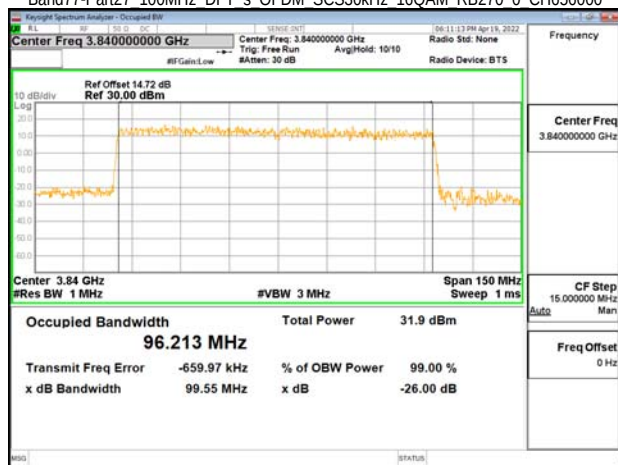
Band77-Part27 100MHz DFT s OFDM SCS30kHz 16QAM RB270 0 CH656000
