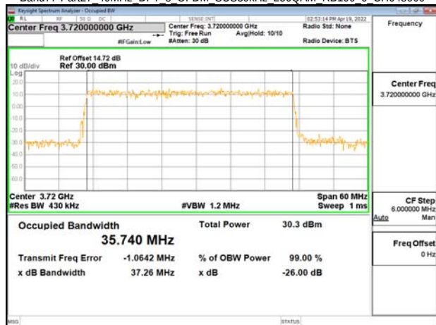
Band77-Part27 40MHz DFT s OFDM SCS30kHz 256QAM RB100 0 CH648000
