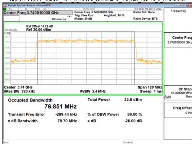
Band77-Part27 80MHz DFT s OFDM SCS30kHz 16QAM RB216 0 CH649334
