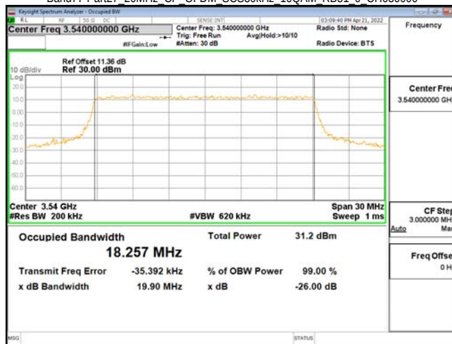
Band77-Part27_20MHz_CP_OFDM_SCS30kHz_16QAM_RB51_0_CH636000
