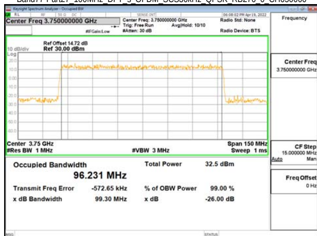
Band77-Part27 100MHz DFT s OFDM SCS30kHz QPSK RB270 0 CH650000
