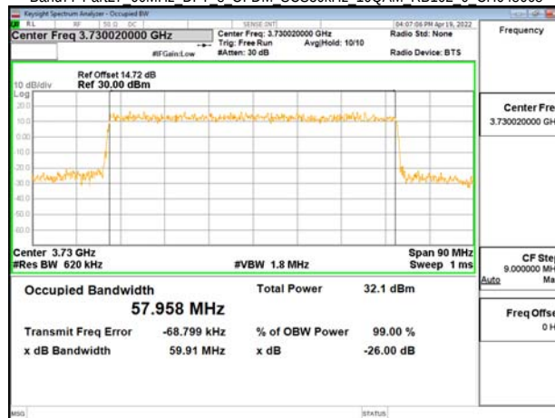
Band77-Part27 60MHz DFT s OFDM SCS30kHz 16QAM RB162 0 CH648668
