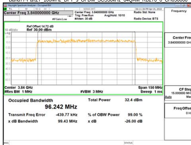
Band77-Part27 100MHz DFT s OFDM SCS30kHz 64QAM RB270 0 CH656000
