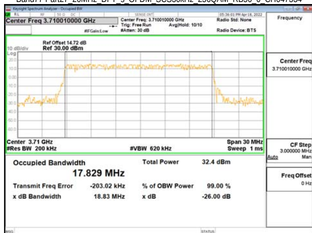
Band77-Part27 20MHz DFT s OFDM SCS30kHz 256OAM RB50 0 CH647334
