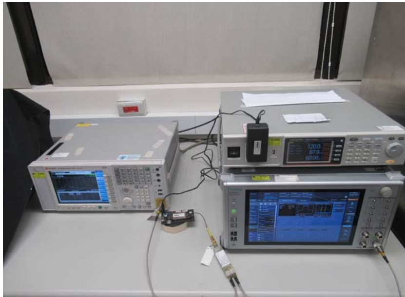
Conducted Setup Photo (Measurement at Antenna Port)
